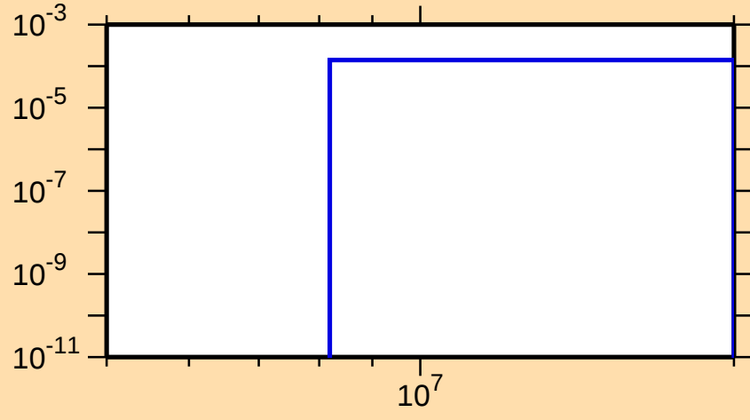
\sigma vs. E for ^{86}\text{Y}(n,t)
