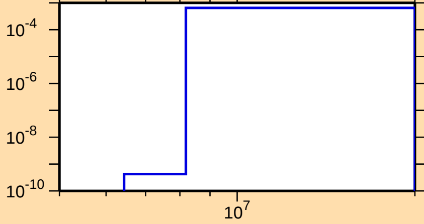
\sigma vs. E for ^{86}\text{Y}(n,p\alpha)
