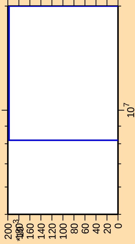
\Delta\sigma/\sigma vs. E for ^{86}\text{Y}(\text{mt117})
