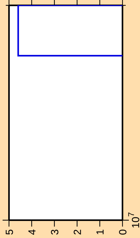
\Delta\sigma/\sigma vs. E for ^{87}\text{Y}(\text{n},\text{nt})
