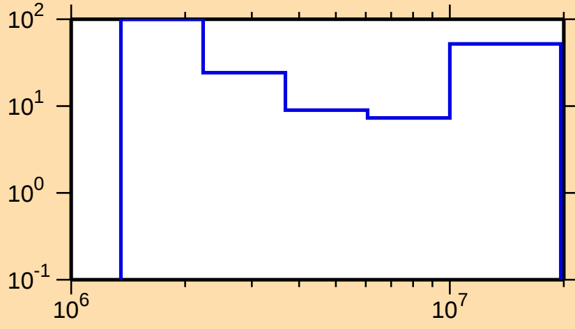
\Delta\sigma/\sigma vs. E for ^{87}\text{Y}(n,n\text{cont.})
