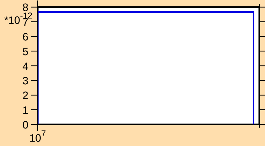
\sigma vs. E for ^{87}\text{Y}(\text{n},\text{pd})
