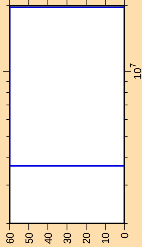
\Delta\sigma/\sigma vs. E for ^{87}\text{Y}(n,d)
