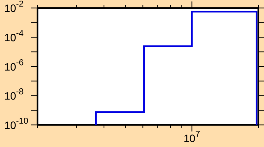
\sigma vs. E for ^{87}\text{Y}(n,d)
