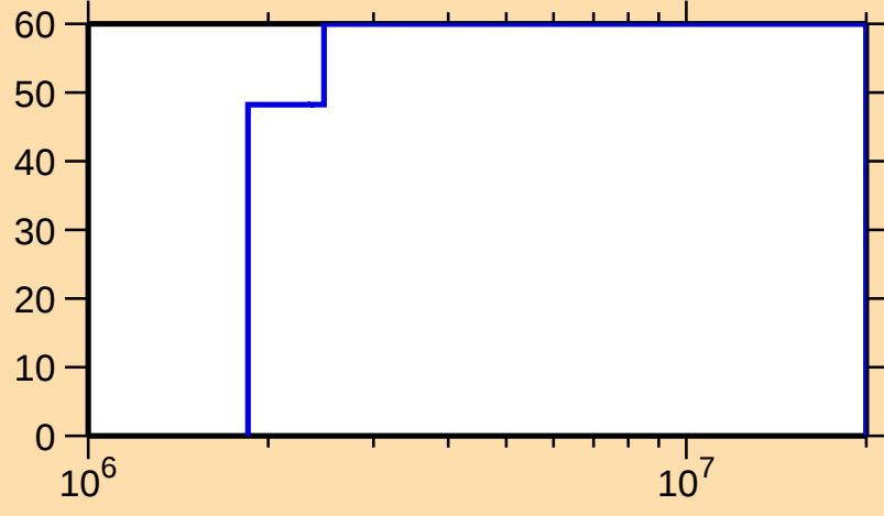
\Delta\sigma/\sigma vs. E for ^{87}\text{Y}(n,n_1)
