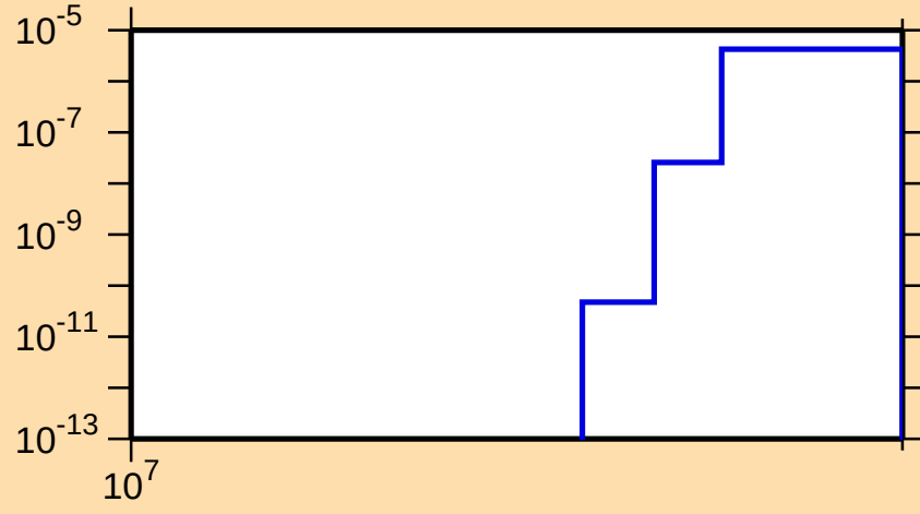
\sigma vs. E for ^{94}\text{Y}(n,\text{nt})
