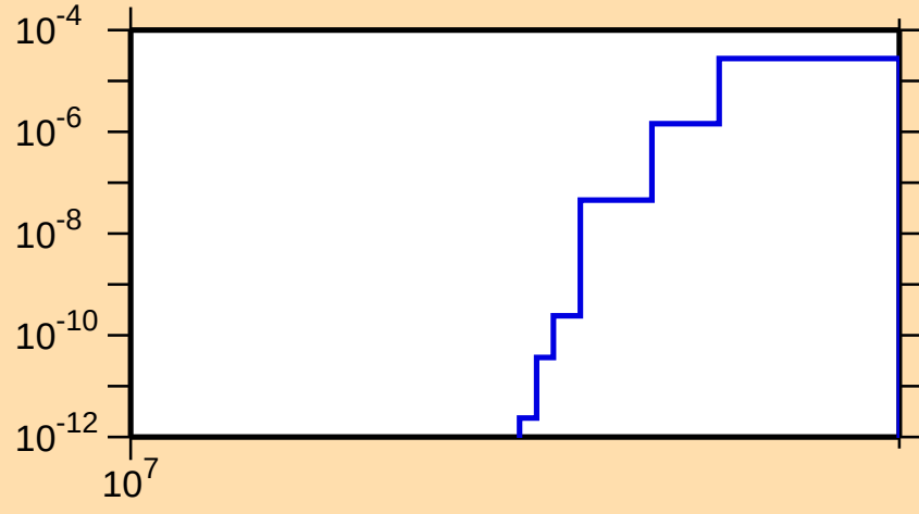
\sigma vs. E for ^{94}\text{Y}(n,\text{nd})
