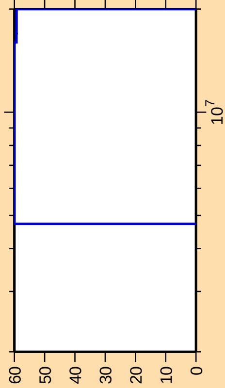
\Delta\sigma/\sigma vs. E for ^{94}\text{Y}(n,p)
