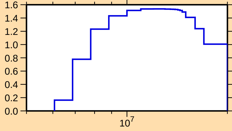
\sigma vs. E for ^{94}\text{Y}(n,2n)
