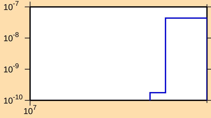
\sigma vs. E for ^{94}\text{Y}(n,2n\alpha)
