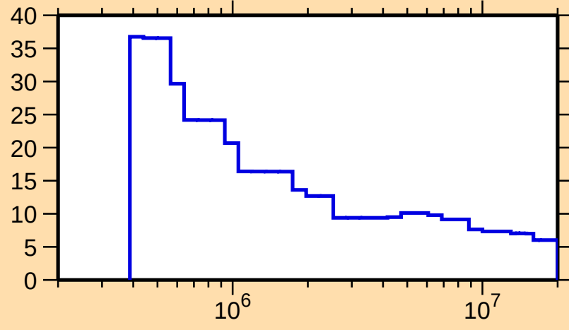
\Delta\sigma/\sigma vs. E for ^{94}\text{Y}(n,\text{nonel.})
