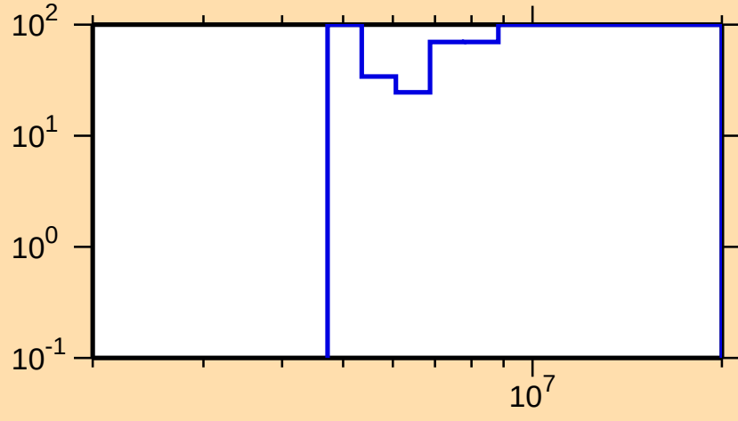
\Delta\sigma/\sigma vs. E for ^{94}\text{Y}(n,n\text{cont.})
