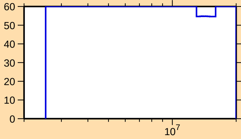
\Delta\sigma/\sigma vs. E for ^{94}\text{Y}(n,\gamma)
