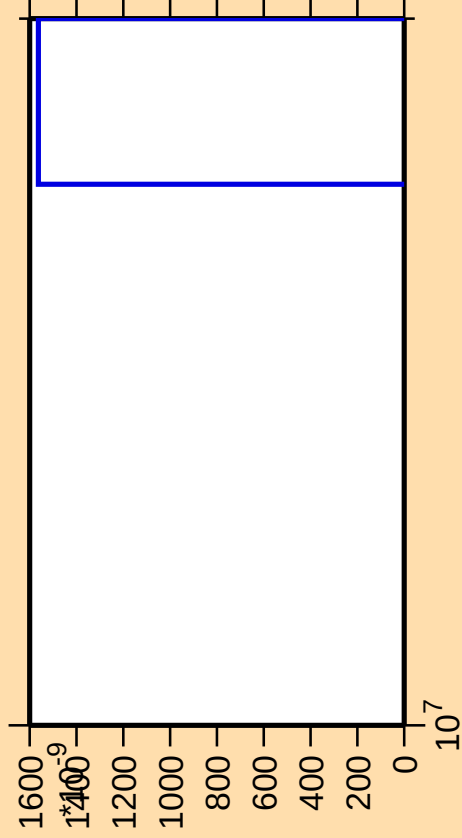
\Delta\sigma/\sigma vs. E for ^{94}\text{Y}(n,3n\alpha)
