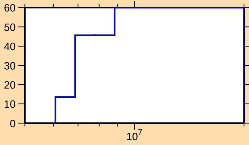
\Delta\sigma/\sigma vs. E for ^{94}\text{Y}(n,\text{inel.})
