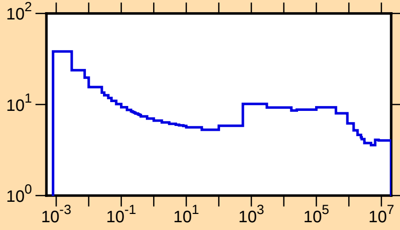
\sigma vs. E for ^{94}\text{Y}(n,\text{tot.})
