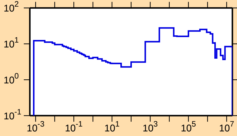
\Delta\sigma/\sigma vs. E for ^{94}\text{Y}(n,\text{tot.})
