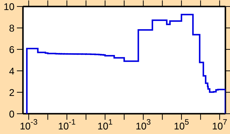
\sigma vs. E for ^{94}\text{Y}(\text{n},\text{el.})
