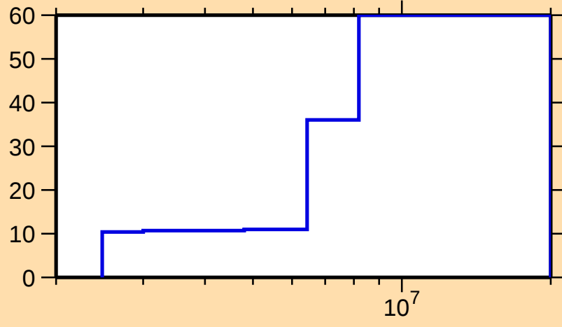
\Delta\sigma/\sigma vs. E for ^{94}\text{Y}(n,\text{inel.})
