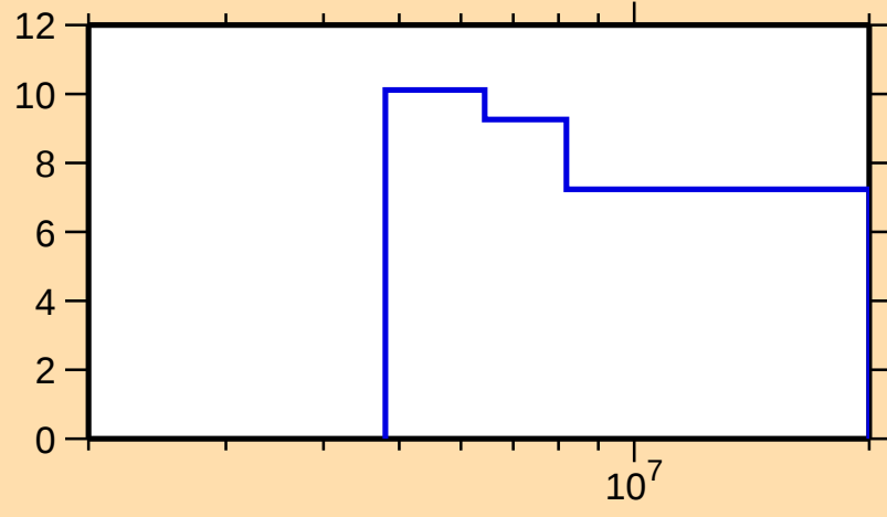
\Delta\sigma/\sigma vs. E for ^{94}\text{Y}(n,\text{nonel.})
