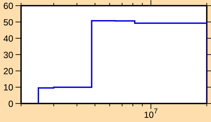
\Delta\sigma/\sigma vs. E for ^{94}\text{Y}(n,n_1)
