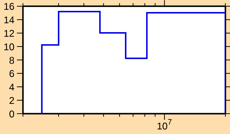
\Delta\sigma/\sigma vs. E for ^{94}\text{Y}(n,\text{el.})
