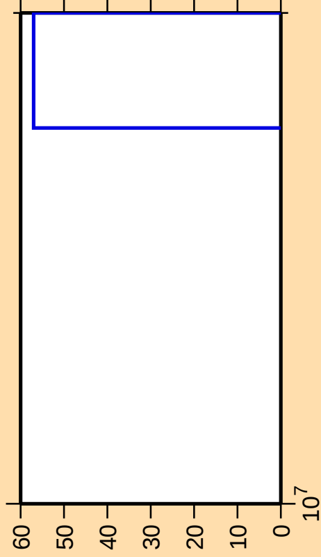
\Delta\sigma/\sigma vs. E for ^{99}\text{Y}(\text{n},2\text{np})
