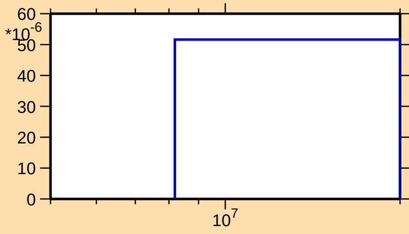
\sigma vs. E for ^{99}\text{Y}(\text{n,d})
