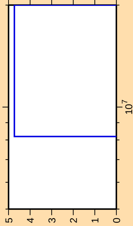
\Delta\sigma/\sigma vs. E for ^{99}\text{Y}(n,2n\alpha)
