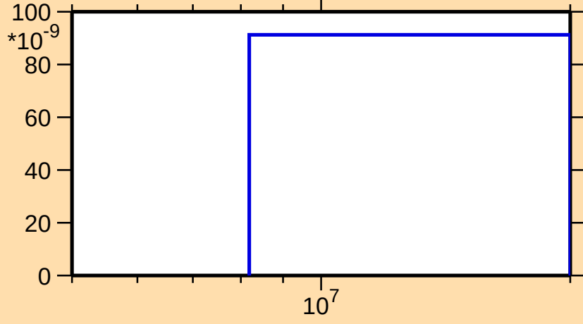
\sigma vs. E for ^{99}\text{Y}(\text{n},\text{nt})
