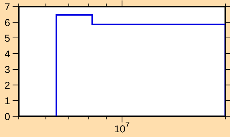
\Delta\sigma/\sigma vs. E for ^{99}\text{Y}(n,\text{nonel.})
