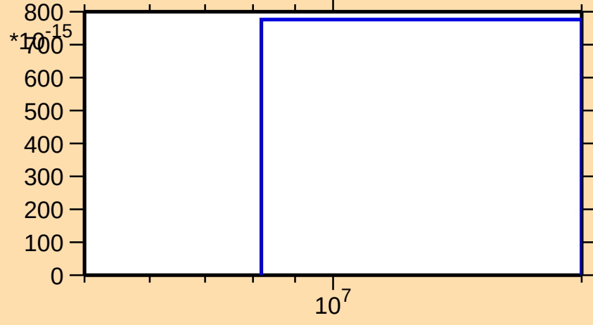
\sigma vs. E for ^{99}\text{Y}(n,2np)
