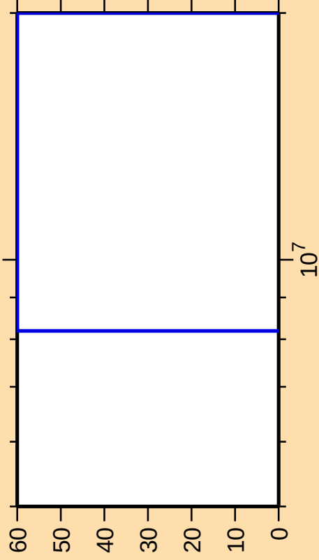
\Delta\sigma/\sigma vs. E for ^{99}\text{Y}(\text{n,d})
