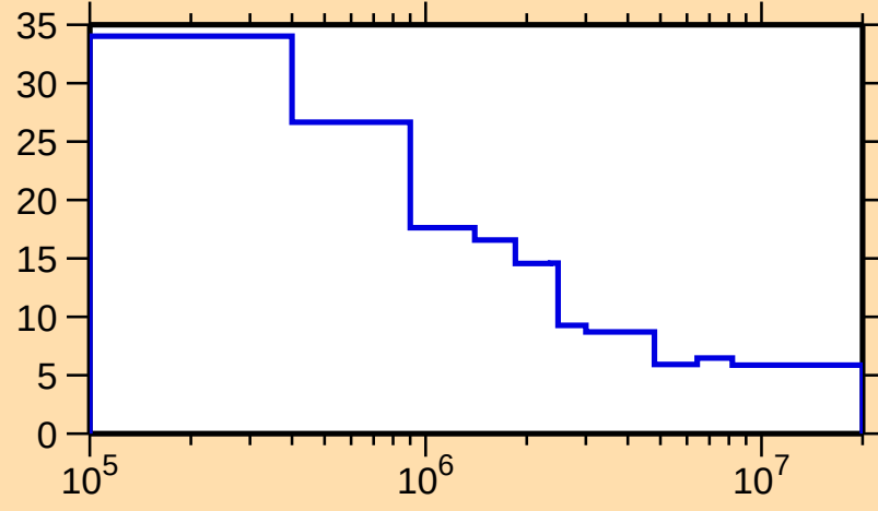
\Delta\sigma/\sigma vs. E for ^{99}\text{Y}(\text{n,nonel.})
