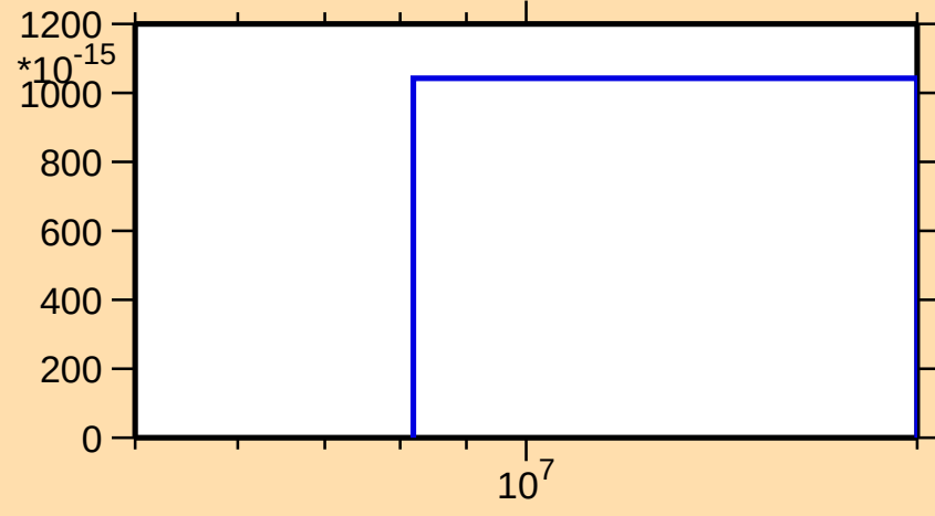
\sigma vs. E for ^{99}\text{Y}(n,2n\alpha)
