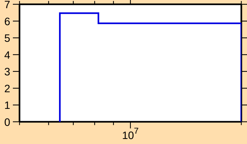
\Delta\sigma/\sigma vs. E for ^{99}\text{Y}(\text{n,nonel.})
