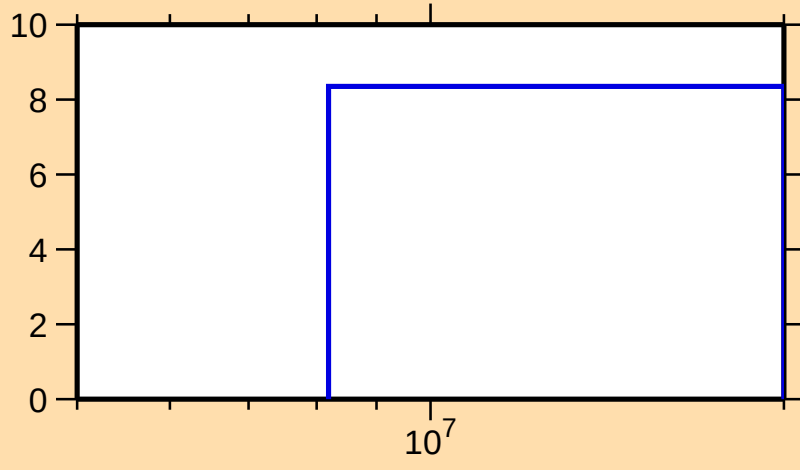
\Delta\sigma/\sigma vs. E for ^{99}\text{Y}(n,\text{tot.})
