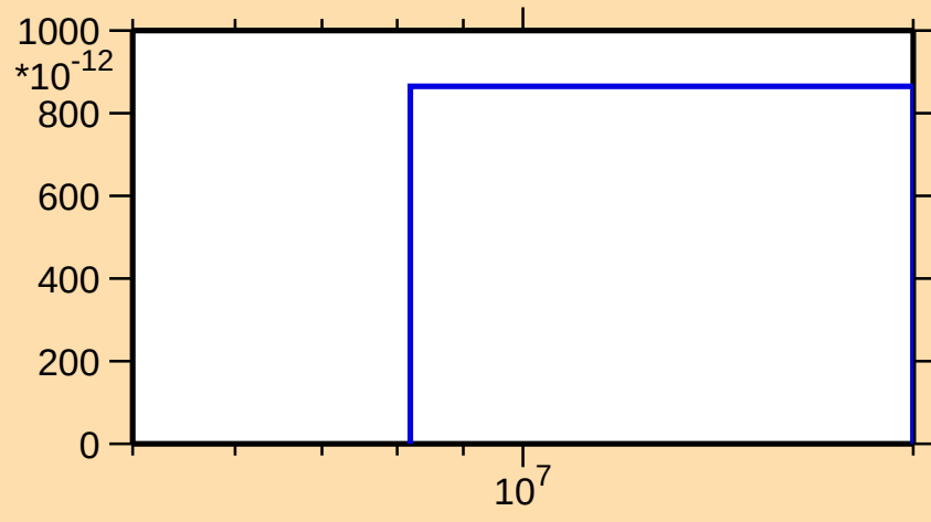
\sigma vs. E for ^{99}\text{Y}(\text{n},\text{nd})
