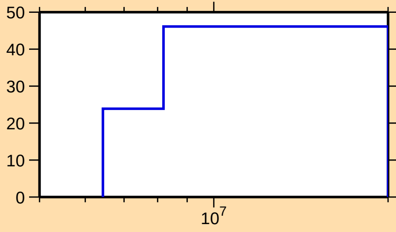
\Delta\sigma/\sigma vs. E for ^{99}\text{Y}(\text{n,inel.})
