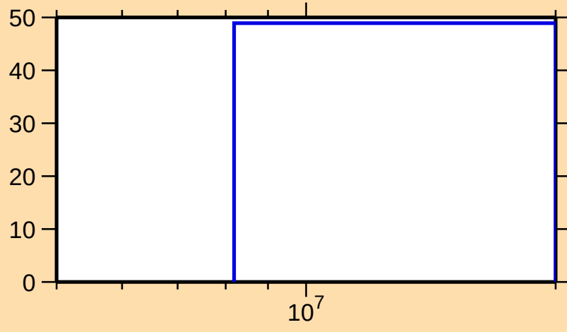
\Delta\sigma/\sigma vs. E for ^{99}\text{Y}(n,\text{ncont.})
