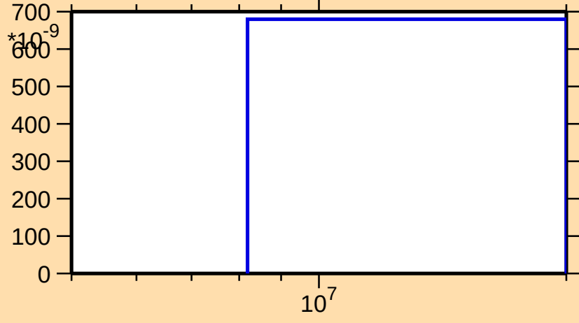
\sigma vs. E for ^{99}\text{Y}(n,n\alpha)
