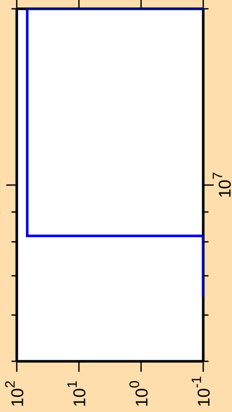
\Delta\sigma/\sigma vs. E for ^{99}\text{Y}(n,p)
