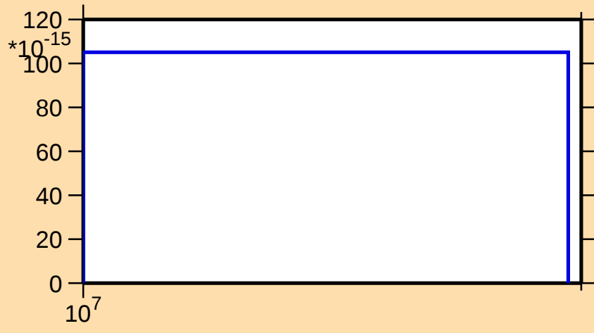
\sigma vs. E for ^{152}\text{Yb}(n,2n\alpha)
