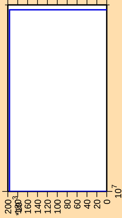
\Delta\sigma/\sigma vs. E for ^{152}\text{Yb}(n,2n\alpha)
