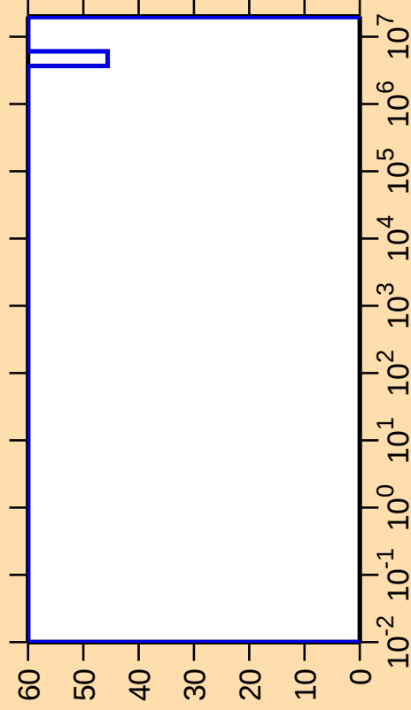
\Delta\sigma/\sigma vs. E for ^{152}\text{Yb}(n,\alpha)
