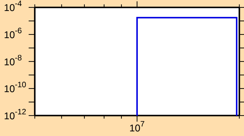
\sigma vs. E for ^{152}\text{Yb}(n,t)
