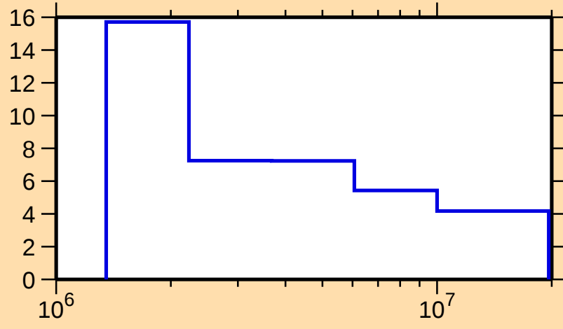
\Delta\sigma/\sigma vs. E for ^{152}\text{Yb}(n,\text{nonel.})
