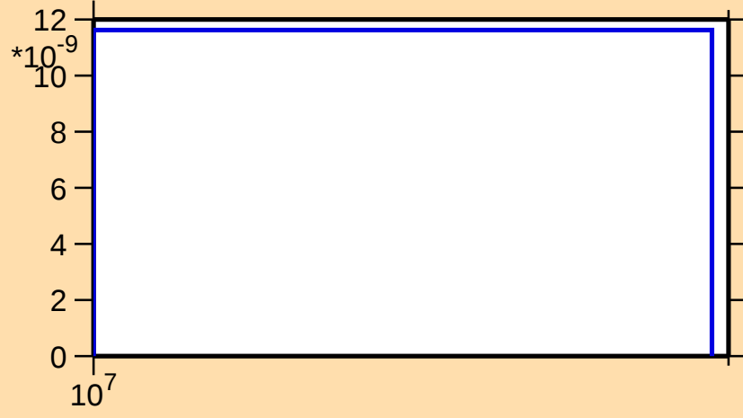
\sigma vs. E for ^{152}\text{Yb}(n,2np)
