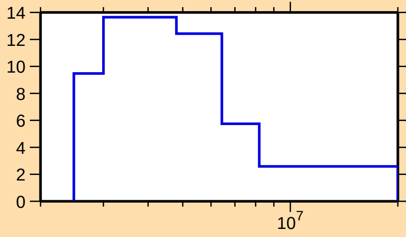
\Delta\sigma/\sigma vs. E for ^{152}\text{Yb}(n,\text{tot.})
