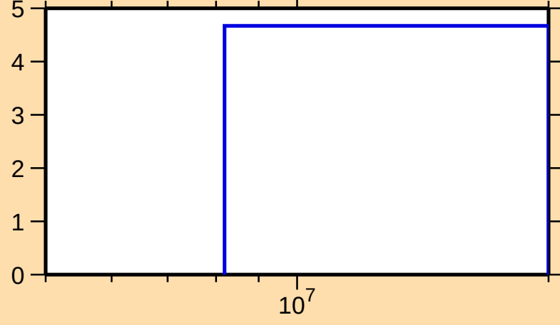
\Delta\sigma/\sigma vs. E for ^{152}\text{Yb}(n,\text{el.})
