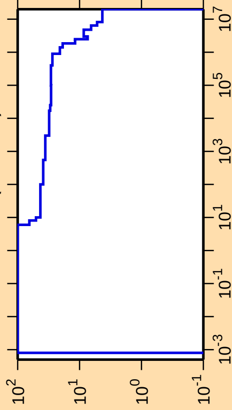
\Delta\sigma/\sigma vs. E for ^{152}\text{Yb}(n,\text{nonel.})
