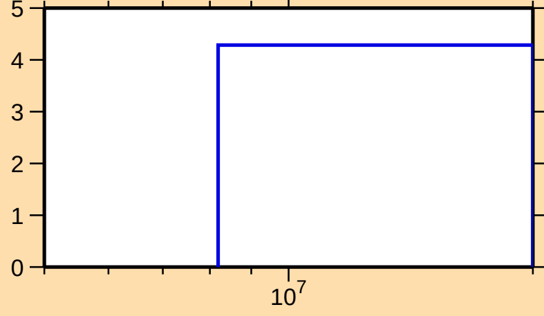
\Delta\sigma/\sigma vs. E for ^{152}\text{Yb}(n,\text{nonel.})
