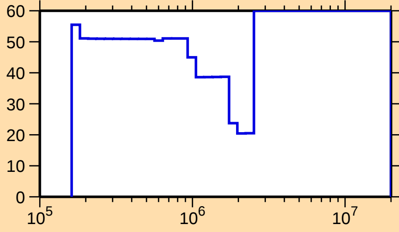
\Delta\sigma/\sigma vs. E for ^{155}\text{Yb}(n,n_1)
