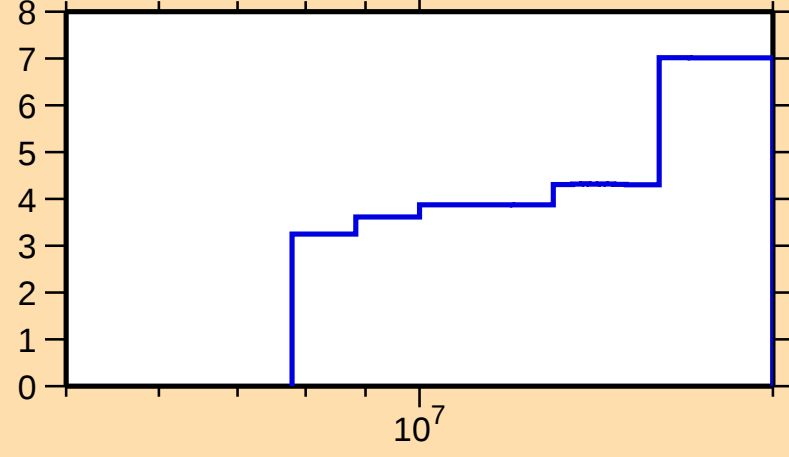
\Delta\sigma/\sigma vs. E for ^{155}\text{Yb}(n,\text{tot.})
