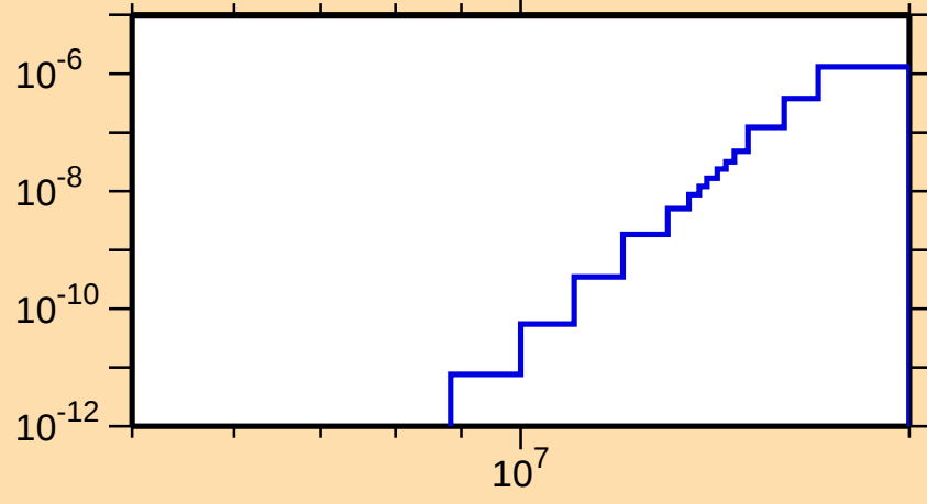
\sigma vs. E for ^{155}\text{Yb}(\text{mt117})
