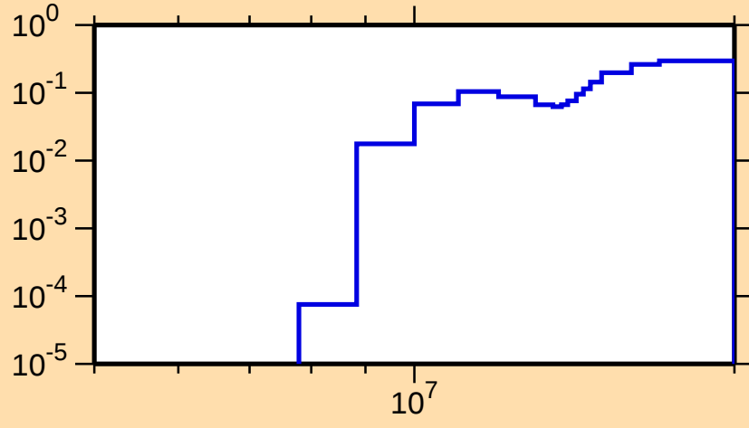
\sigma vs. E for ^{155}\text{Yb}(n,2n)
