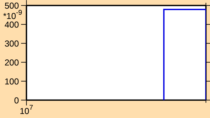
\sigma vs. E for ^{155}\text{Yb}(n,3n)
