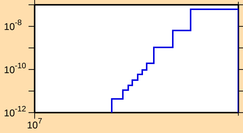
\sigma vs. E for ^{155}\text{Yb} (mt 34)
