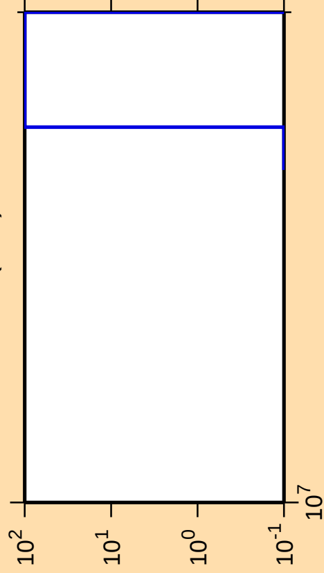
\Delta\sigma/\sigma vs. E for ^{155}\text{Yb}(n,nt)
