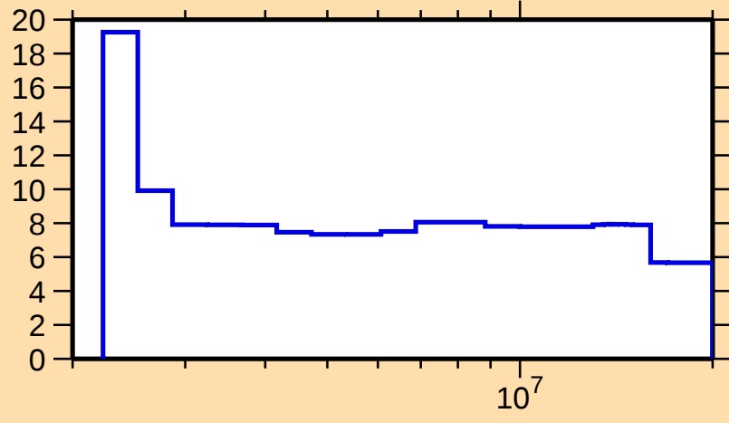
\Delta\sigma/\sigma vs. E for ^{155}\text{Yb}(n,\text{nonel.})
