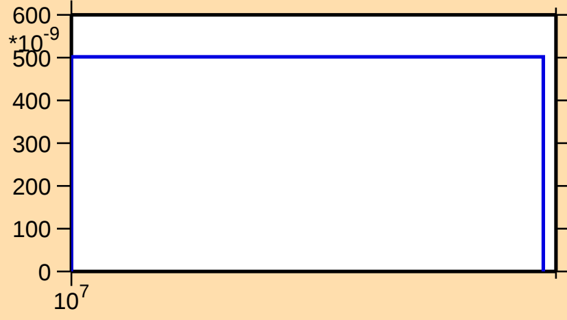
\sigma vs. E for ^{155}\text{Yb}(n,\text{nd})
