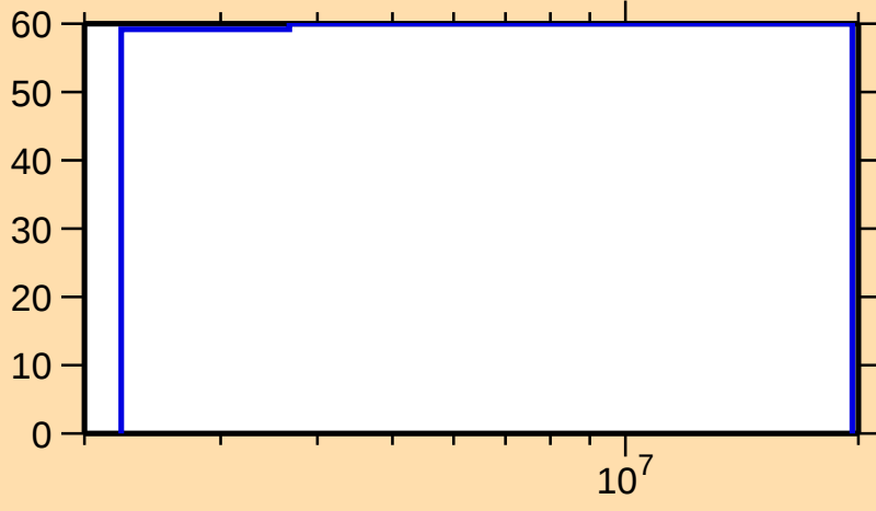
\Delta\sigma/\sigma vs. E for ^{155}\text{Yb}(n,n_1)
