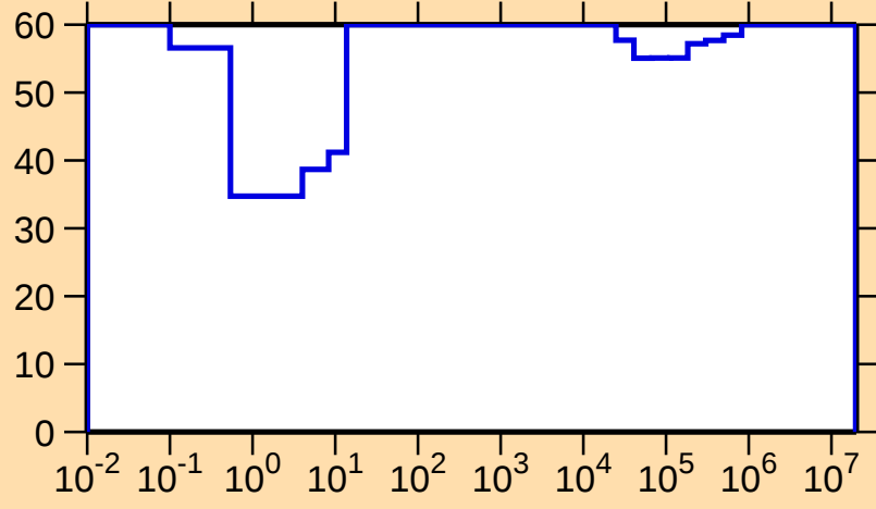
\Delta\sigma/\sigma vs. E for ^{155}\text{Yb}(n,\gamma)
