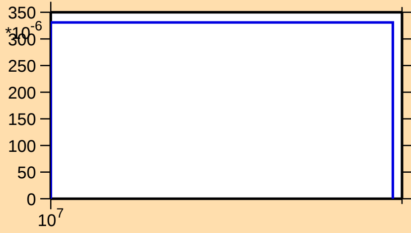
\sigma vs. E for ^{155}\text{Yb}(n,2np)
