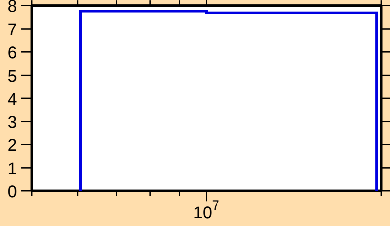
\Delta\sigma/\sigma vs. E for ^{155}\text{Yb}(n,\text{nonel.})
