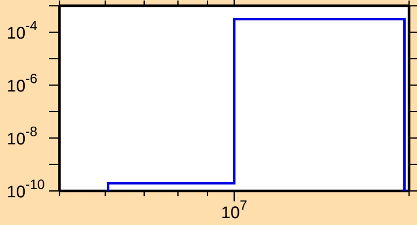
\sigma vs. E for ^{155}\text{Yb}(n,t)
