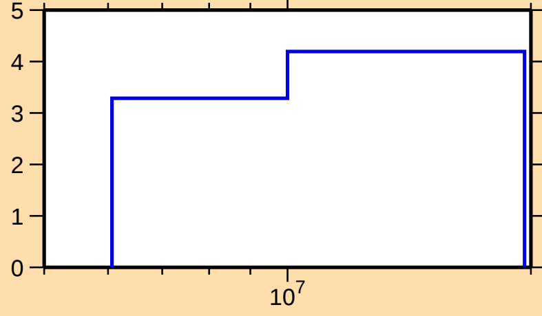
\Delta\sigma/\sigma vs. E for ^{155}\text{Yb}(n,\text{tot.})
