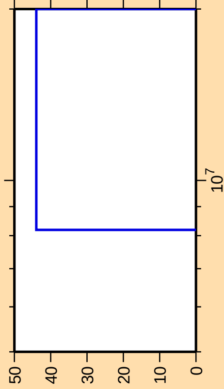
\Delta\sigma/\sigma vs. E for ^{155}\text{Yb}(n,p)
