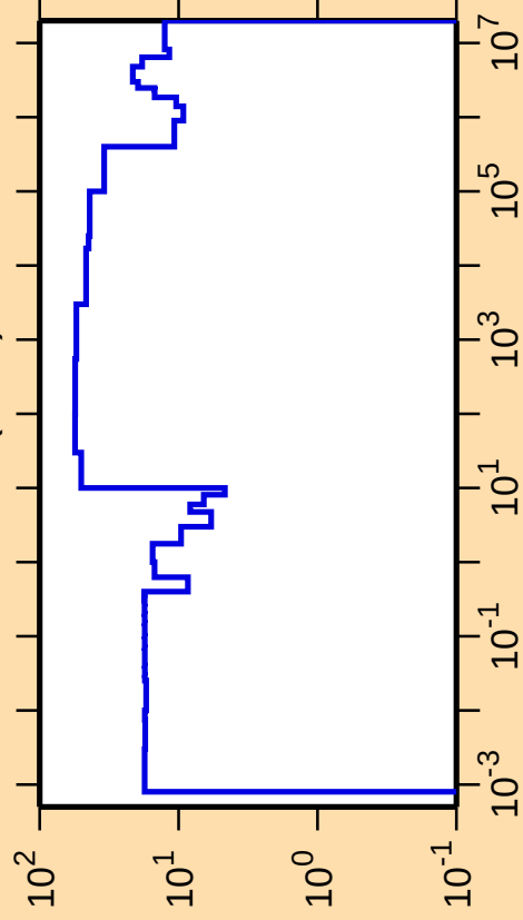
\Delta\sigma/\sigma vs. E for ^{155}\text{Yb}(n,\text{el.})
