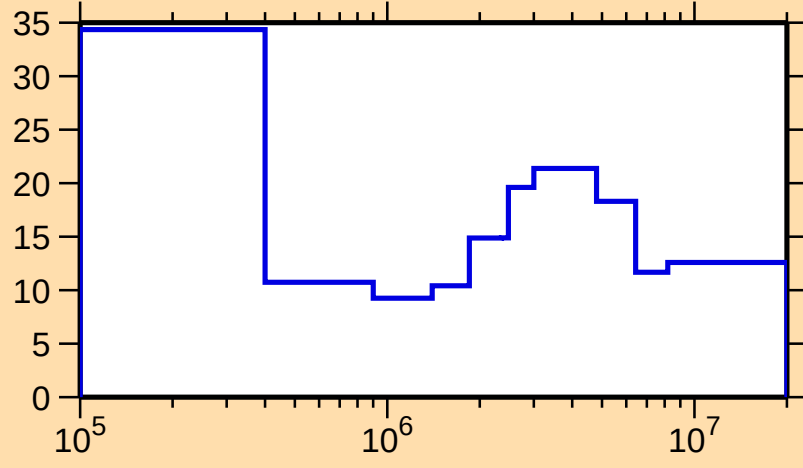
\Delta\sigma/\sigma vs. E for ^{155}\text{Yb}(n,\text{el.})
