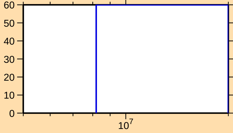
\Delta\sigma/\sigma vs. E for ^{155}\text{Yb}(n,2n)
