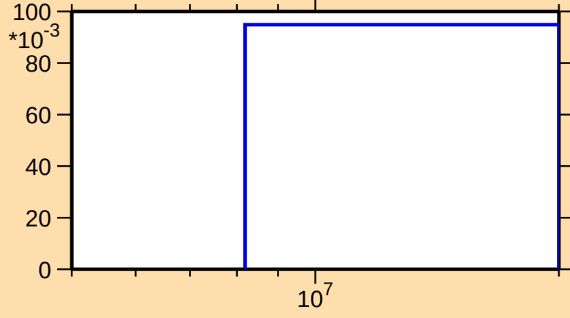
\sigma vs. E for ^{155}\text{Yb}(n,2n)
