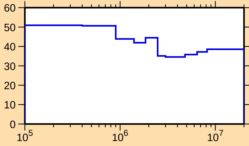
\Delta\sigma/\sigma vs. E for ^{155}\text{Yb}(n,\text{inel.})
