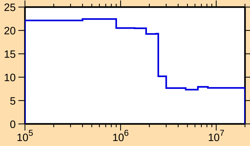
\Delta\sigma/\sigma vs. E for ^{155}\text{Yb}(n,\text{nonel.})
