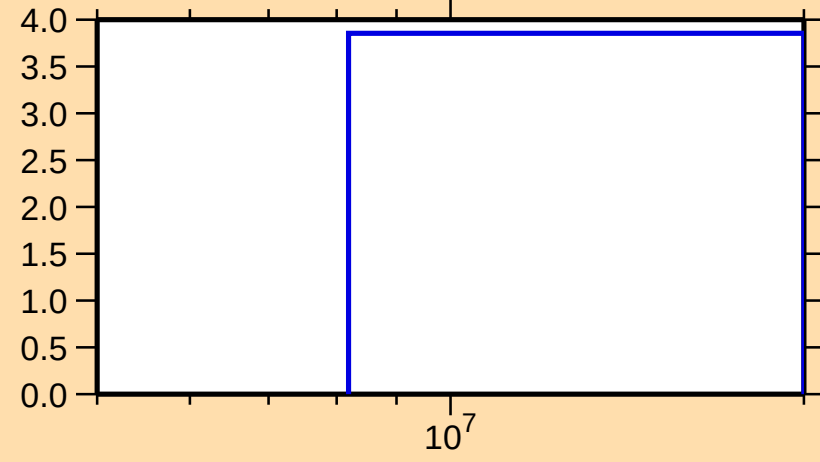
\Delta\sigma/\sigma vs. E for ^{155}\text{Yb}(n,\text{tot.})
