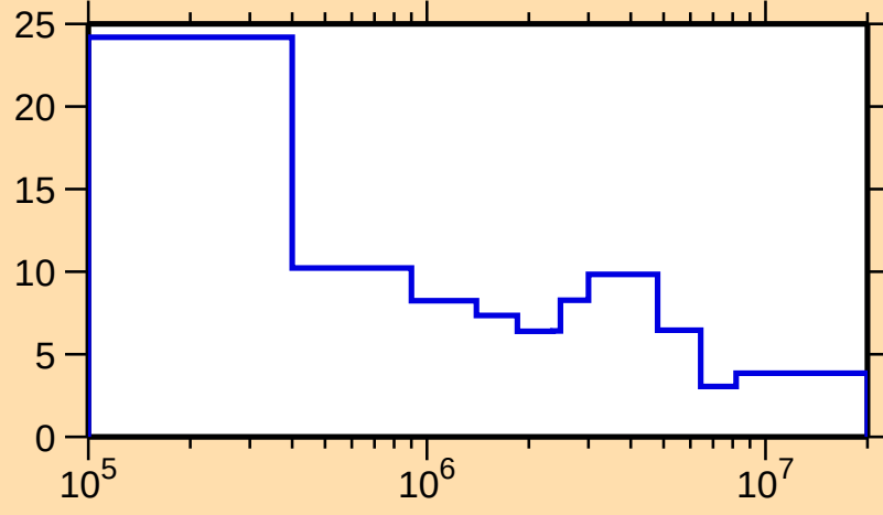
\Delta\sigma/\sigma vs. E for ^{155}\text{Yb}(n,\text{tot.})
