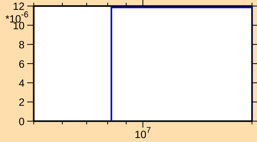
\sigma vs. E for ^{155}\text{Yb}(n,\text{pd})
