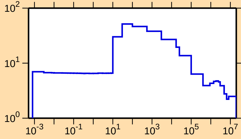
\sigma vs. E for ^{155}\text{Yb}(n,\text{el.})
