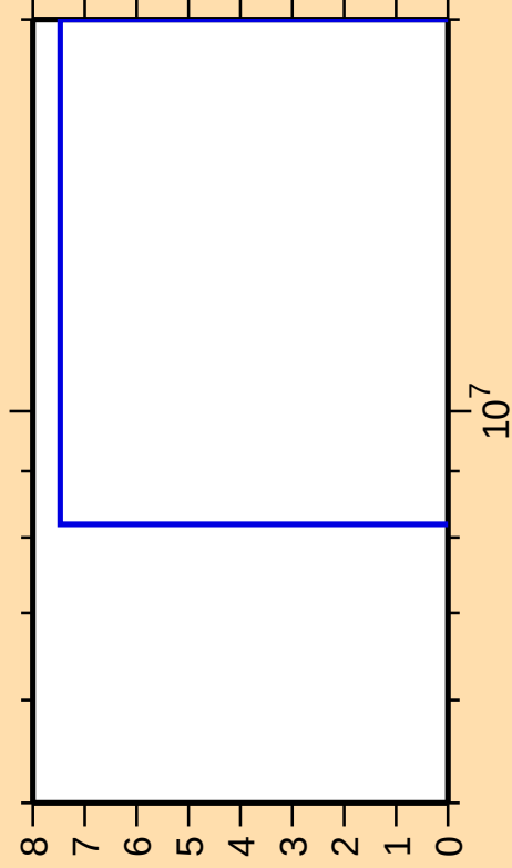
\Delta\sigma/\sigma vs. E for ^{155}\text{Yb}(n,nt)
