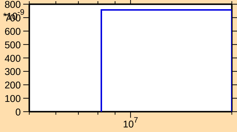
\sigma vs. E for ^{155}\text{Yb}(n,\text{pt})
