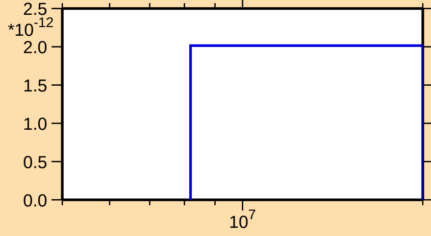
\sigma vs. E for ^{155}\text{Yb}(n,nt)
