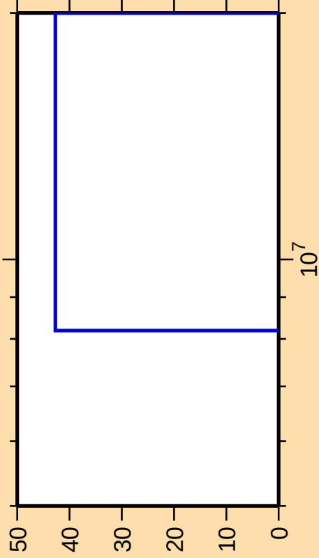
\Delta\sigma/\sigma vs. E for ^{155}\text{Yb}(n,n\text{cont.})
