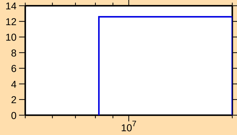
\Delta\sigma/\sigma vs. E for ^{155}\text{Yb}(n,\text{el.})
