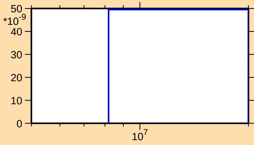
\sigma vs. E for ^{155}\text{Yb}(\text{mt117})
