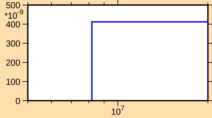
\sigma vs. E for ^{155}\text{Yb}(n,\text{nd})
