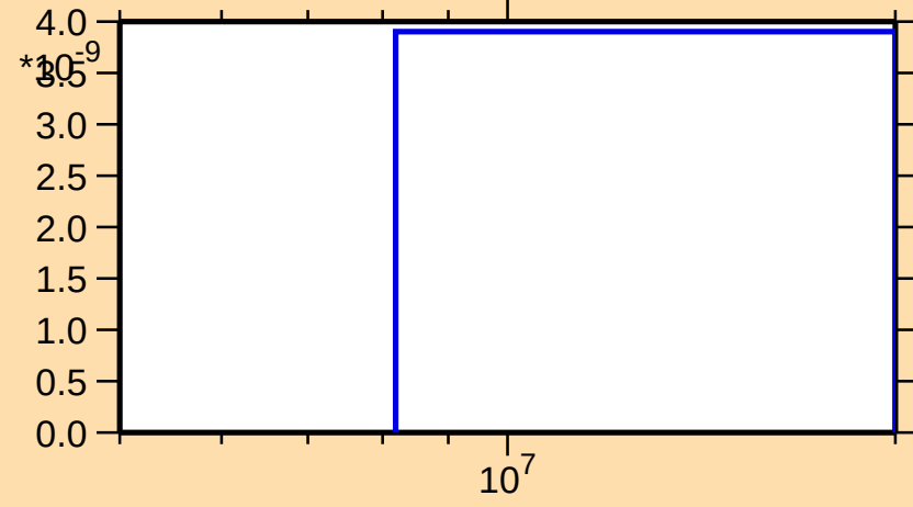
\sigma vs. E for ^{155}\text{Yb}(n,3n)
