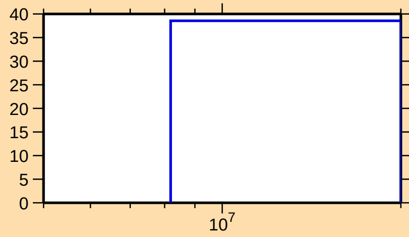
\Delta\sigma/\sigma vs. E for ^{155}\text{Yb}(n,\text{inel.})
