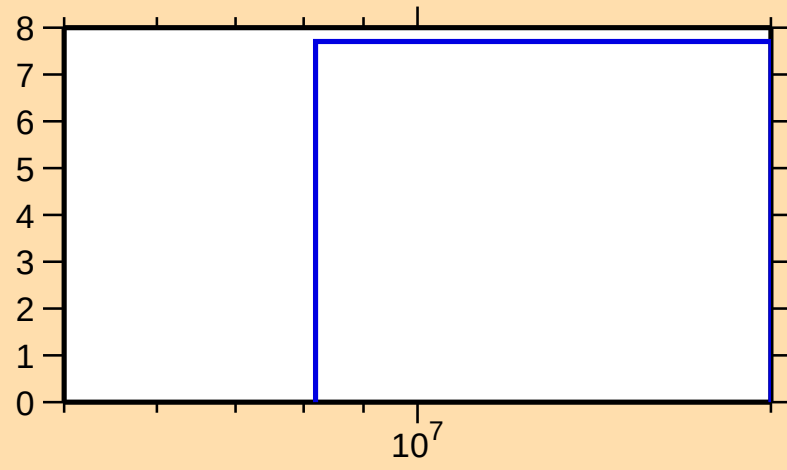
\Delta\sigma/\sigma vs. E for ^{155}\text{Yb}(n,\text{nonel.})
