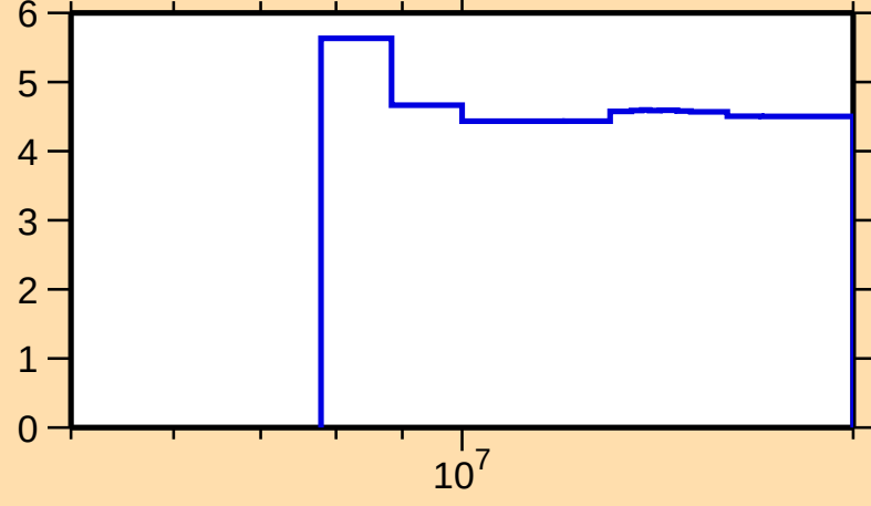
\Delta\sigma/\sigma vs. E for ^{161}\text{Yb}(n,\text{nonel.})
