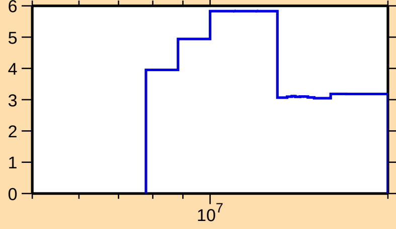
\Delta\sigma/\sigma vs. E for ^{161}\text{Yb}(n,\text{el.})
