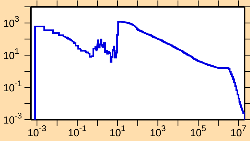
\sigma vs. E for ^{161}\text{Yb}(n,\gamma)
