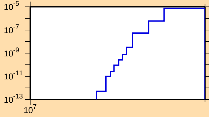
\sigma vs. E for ^{161}\text{Yb}(n,\text{nd})
