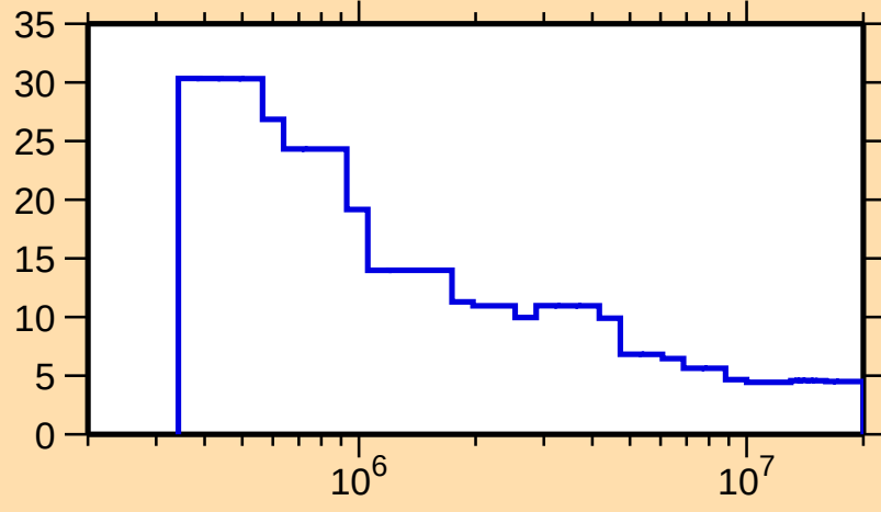
\Delta\sigma/\sigma vs. E for ^{161}\text{Yb}(n,n\text{oncl.})
