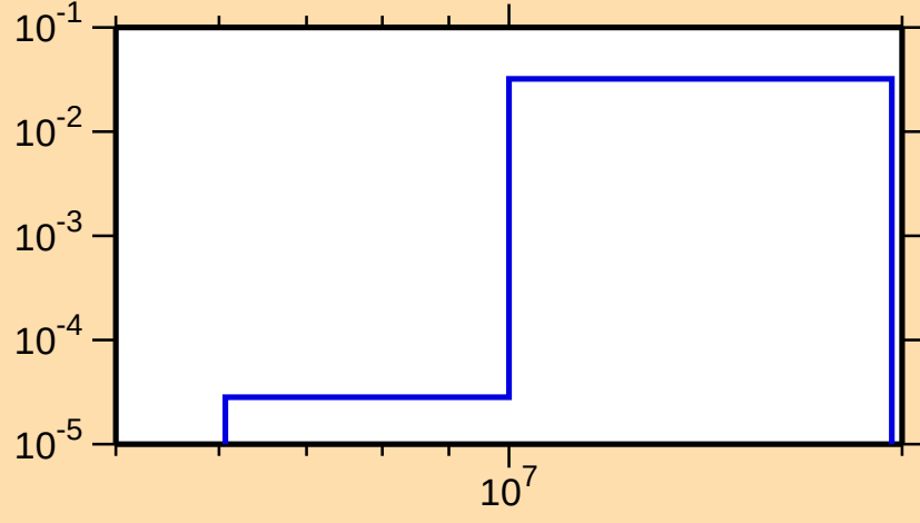
\sigma vs. E for ^{161}\text{Yb}(n,np)
