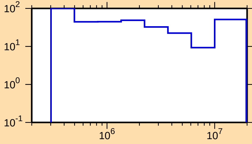
\Delta\sigma/\sigma vs. E for ^{161}\text{Yb}(n,n\text{cont.})
