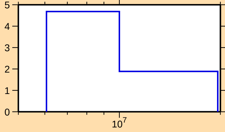
\Delta\sigma/\sigma vs. E for ^{161}\text{Yb}(n,\text{tot.})
