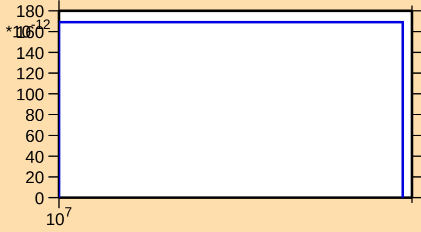
\sigma vs. E for ^{161}\text{Yb}(n,\text{pt})
