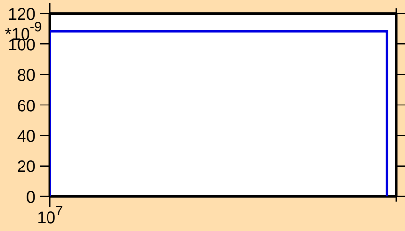
\sigma vs. E for ^{161}\text{Yb}(n,\text{nd})
