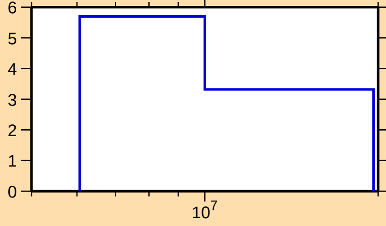
\Delta\sigma/\sigma vs. E for ^{161}\text{Yb}(n,\text{el.})
