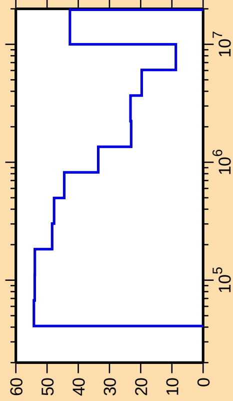
\Delta\sigma/\sigma vs. E for ^{161}\text{Yb}(n,\text{inel.})
