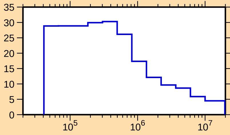
\Delta\sigma/\sigma vs. E for ^{161}\text{Yb}(n,\text{nonel.})
