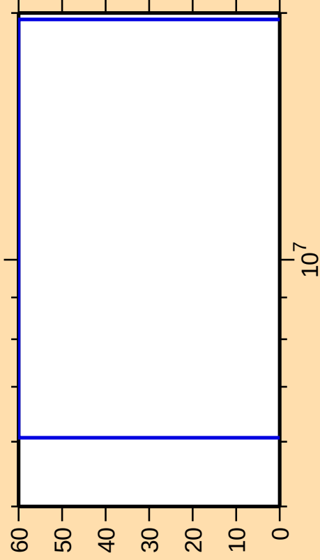
\Delta\sigma/\sigma vs. E for ^{161}\text{Yb}(n,np)
