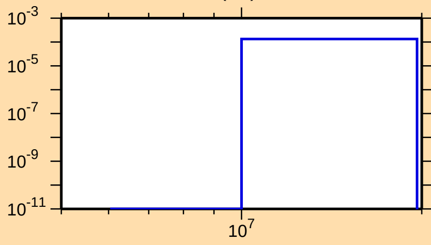
\sigma vs. E for ^{161}\text{Yb}(n,t)
