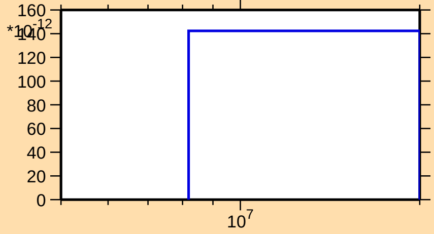
\sigma vs. E for ^{161}\text{Yb} (mt 45)
