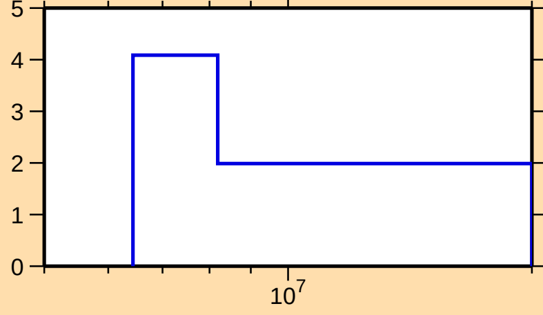
\Delta\sigma/\sigma vs. E for ^{161}\text{Yb}(n,\text{tot.})
