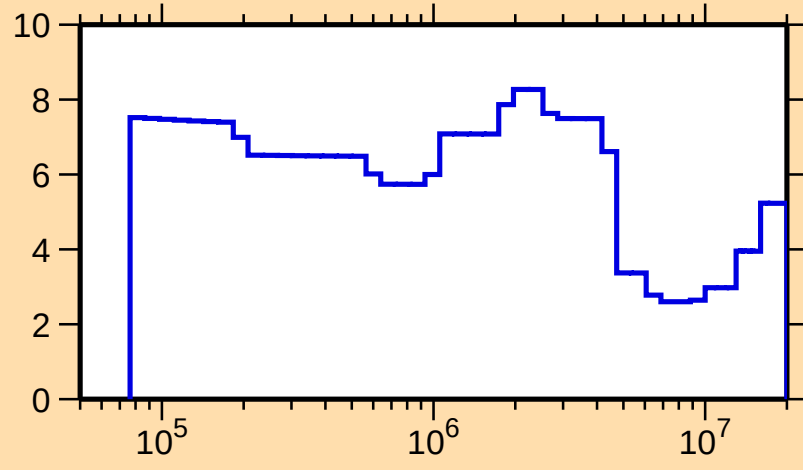
\Delta\sigma/\sigma vs. E for ^{170}\text{Yb}(n,\text{tot.})
