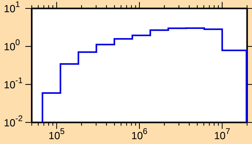
\sigma vs. E for ^{170}\text{Yb}(n,\text{inel.})
