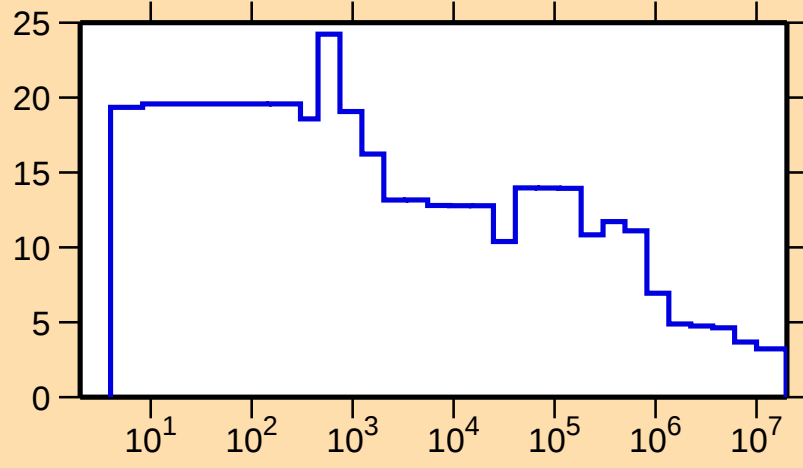
\Delta\sigma/\sigma vs. E for ^{170}\text{Yb}(n,\text{nonel.})
