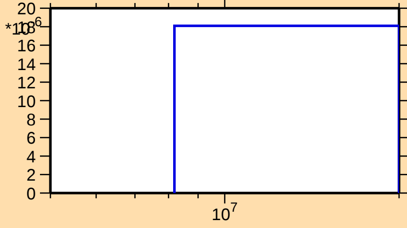
\sigma vs. E for ^{170}\text{Yb}(n,t)
