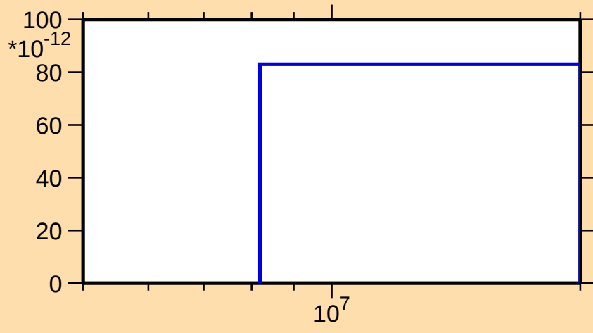
\sigma vs. E for ^{170}\text{Yb}(n,\text{He}3)
