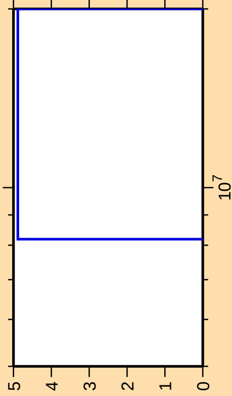
\Delta\sigma/\sigma vs. E for ^{170}\text{Yb}(n,p\alpha)
