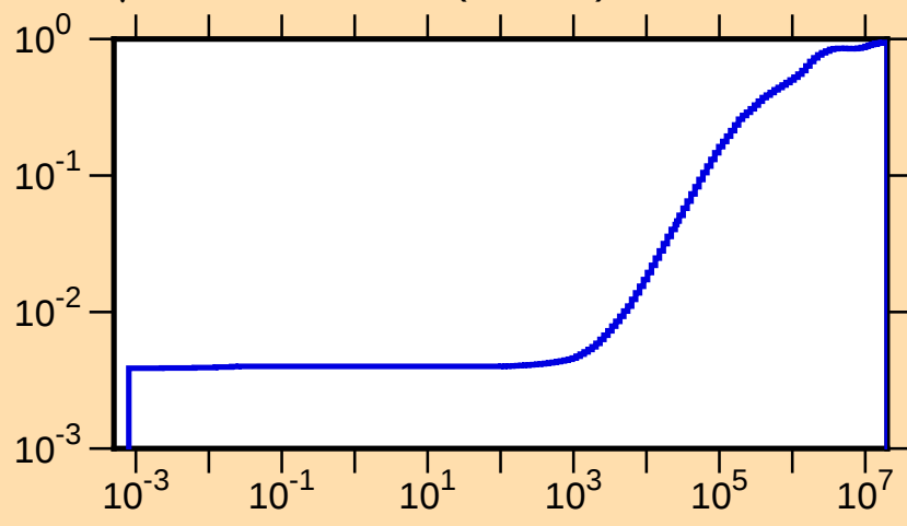
\mu vs. E for ^{174}\text{Yb}(\text{mt251})
