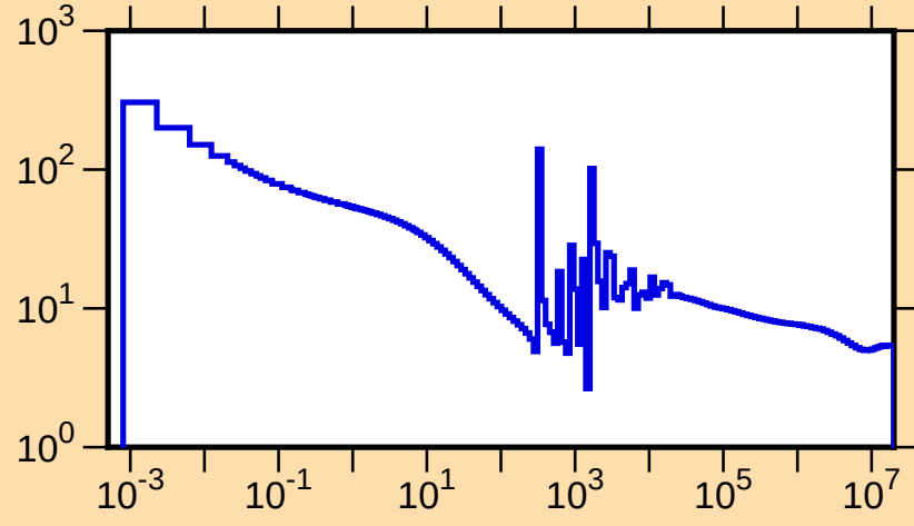
\sigma vs. E for ^{174}\text{Yb}(n,\text{tot.})
