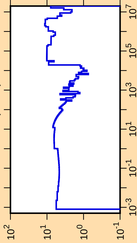
\Delta\sigma/\sigma vs. E for ^{174}\text{Yb}(n,\text{tot.})
