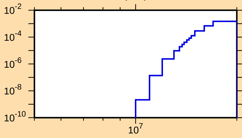
\sigma vs. E for ^{174}\text{Yb}(n,d)
