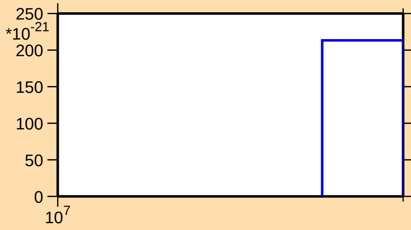
\sigma vs. E for ^{174}\text{Yb} (mt 11)
