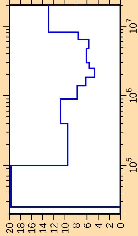
\Delta\sigma/\sigma vs. E for ^{174}\text{Yb}(n,\text{inel.})
