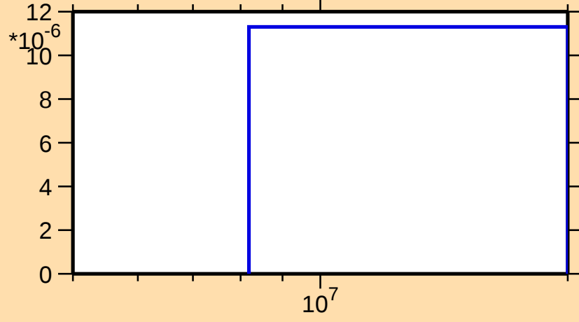
\sigma vs. E for ^{174}\text{Yb}(n,t)
