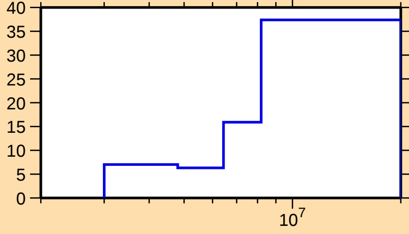
\Delta\sigma/\sigma vs. E for ^{174}\text{Yb}(n,n\text{cont.})
