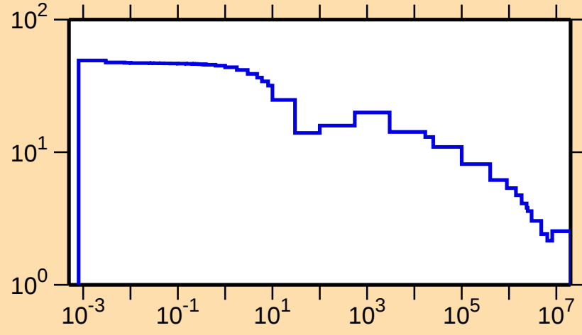
\sigma vs. E for ^{174}\text{Yb}(n,\text{el.})
