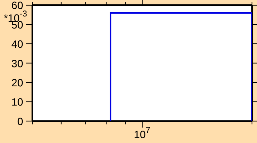
\sigma vs. E for ^{174}\text{Yb}(n,3n)
