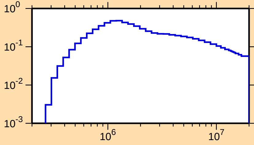
\sigma vs. E for ^{176}\text{Yb}(n,n_2)
