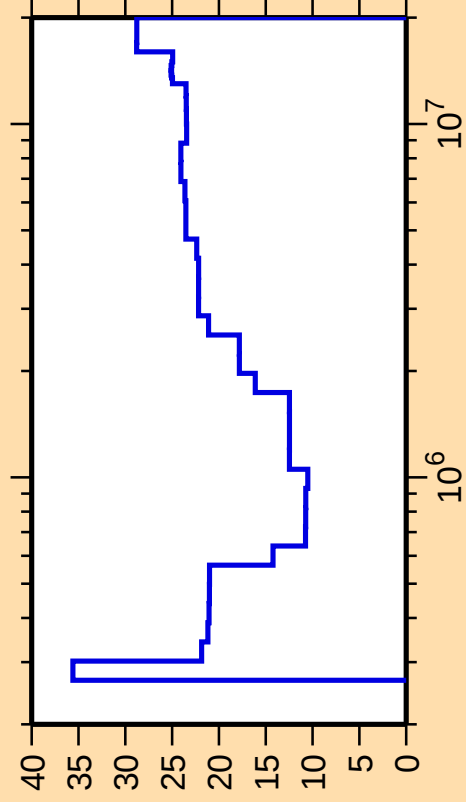
\Delta\sigma/\sigma vs. E for ^{176}\text{Yb}(n,n_2)
