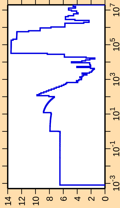
\Delta\sigma/\sigma vs. E for ^{176}\text{Yb}(n,\text{el.})
