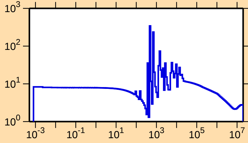
\sigma vs. E for ^{176}\text{Yb}(n,\text{el.})
