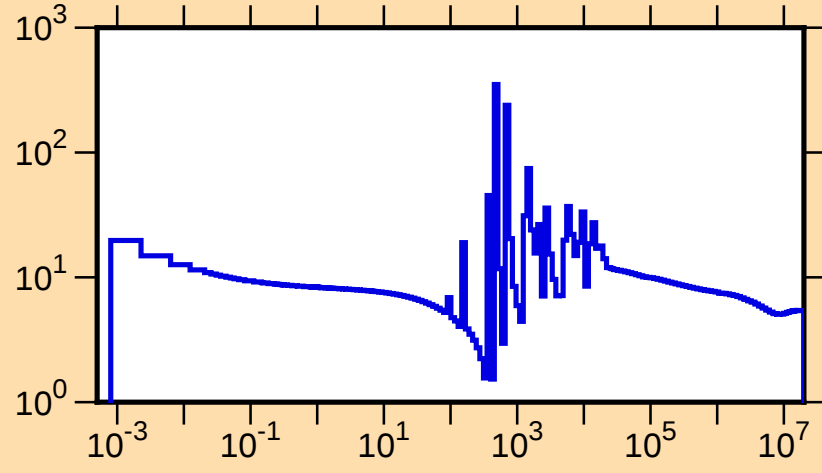
\sigma vs. E for ^{176}\text{Yb}(n,\text{tot.})
