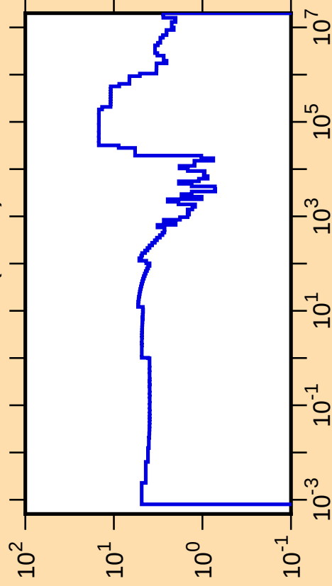
\Delta\sigma/\sigma vs. E for ^{176}\text{Yb}(n,\text{tot.})
