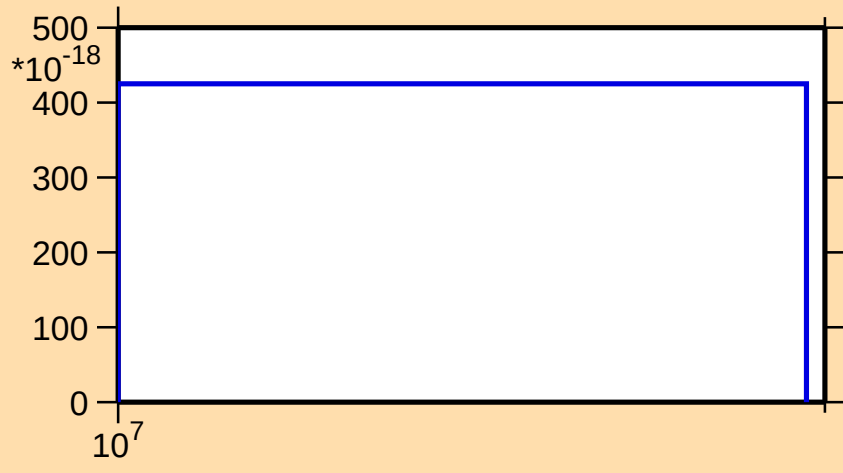
\sigma vs. E for ^{176}\text{Yb}(n,3n\alpha)
