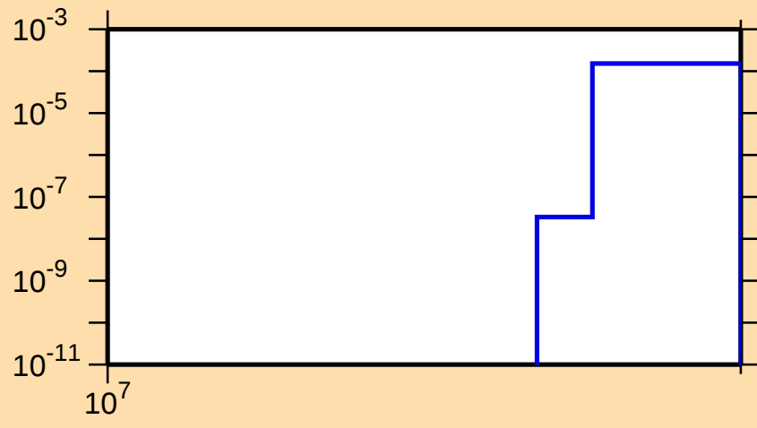
\sigma vs. E for ^{63}\text{Zn}(n,2np)
