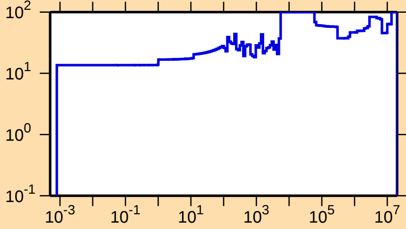
\Delta\sigma/\sigma vs. E for ^{63}\text{Zn}(n,\gamma)
