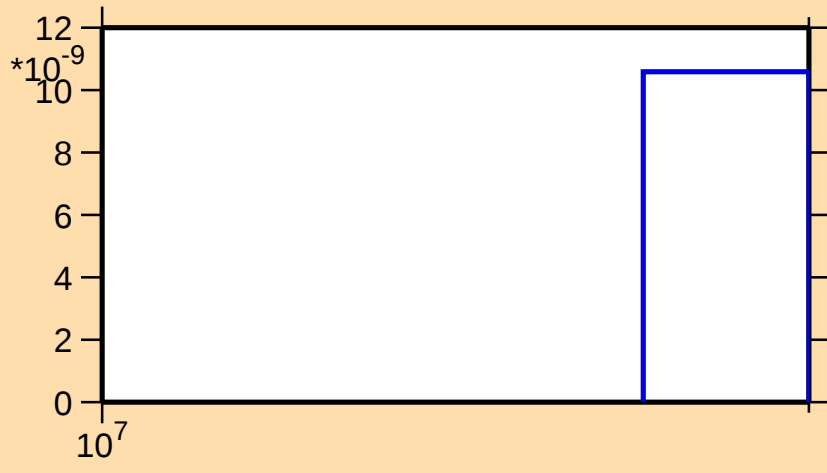
\sigma vs. E for ^{63}\text{Zn}(\text{mt } 45)
