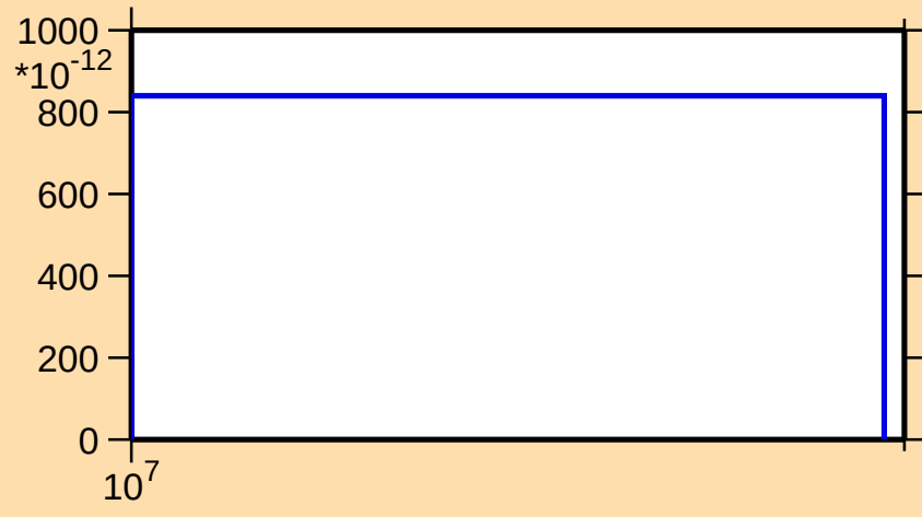
\sigma vs. E for ^{63}\text{Zn}(\text{mt } 34)
