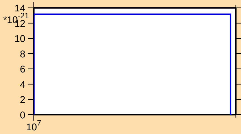
\sigma vs. E for ^{63}\text{Zn}(n,\text{nt})
