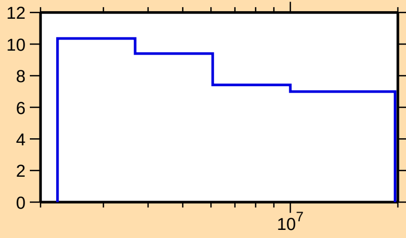
\Delta\sigma/\sigma vs. E for ^{63}\text{Zn}(n,\text{nonel.})
