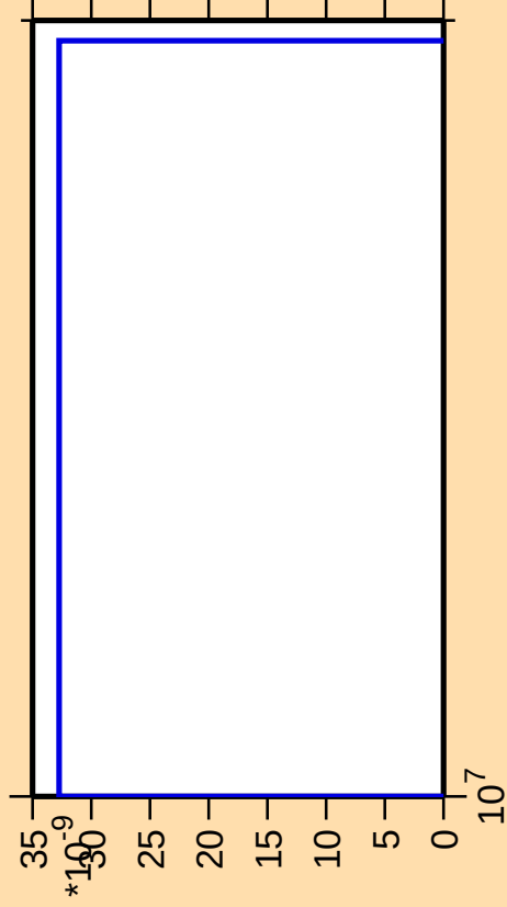
\Delta\sigma/\sigma vs. E for ^{63}\text{Zn}(n,\text{nt})
