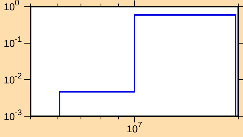
\sigma vs. E for ^{63}\text{Zn}(n,np)
