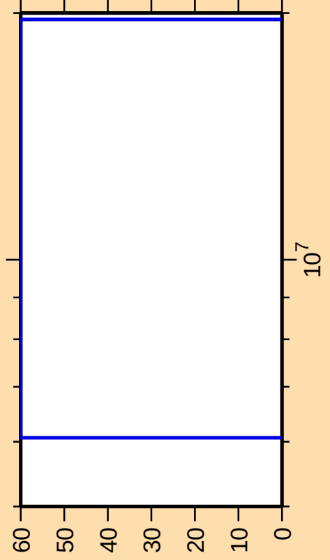
\Delta\sigma/\sigma vs. E for ^{63}\text{Zn}(n,\alpha)
