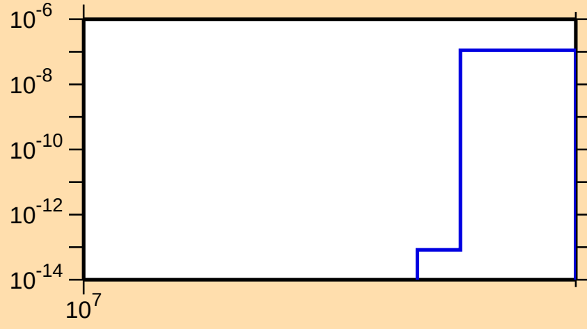
\sigma vs. E for ^{66}\text{Zn}(n,\text{nd})
