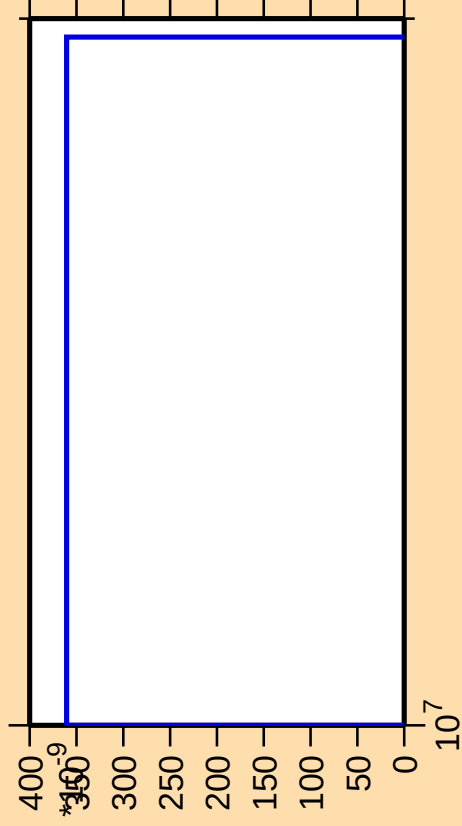
\Delta\sigma/\sigma vs. E for ^{66}\text{Zn}(\text{mt } 34)
