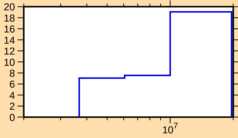
\Delta\sigma/\sigma vs. E for ^{66}\text{Zn}(n,n\text{cont.})
