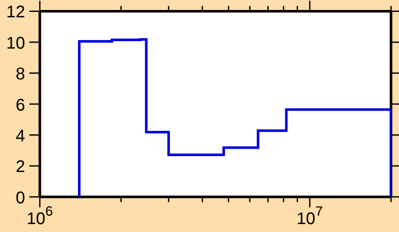
\Delta\sigma/\sigma vs. E for ^{69}\text{Zn}(n,\text{tot.})
