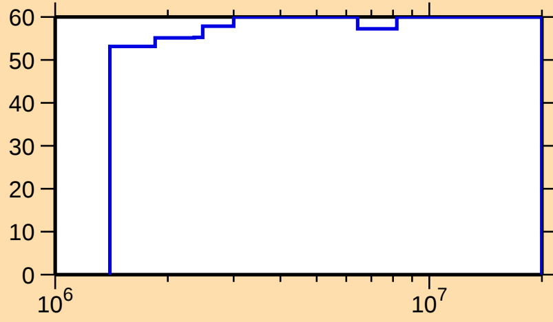
\Delta\sigma/\sigma vs. E for ^{69}\text{Zn}(n,\gamma)
