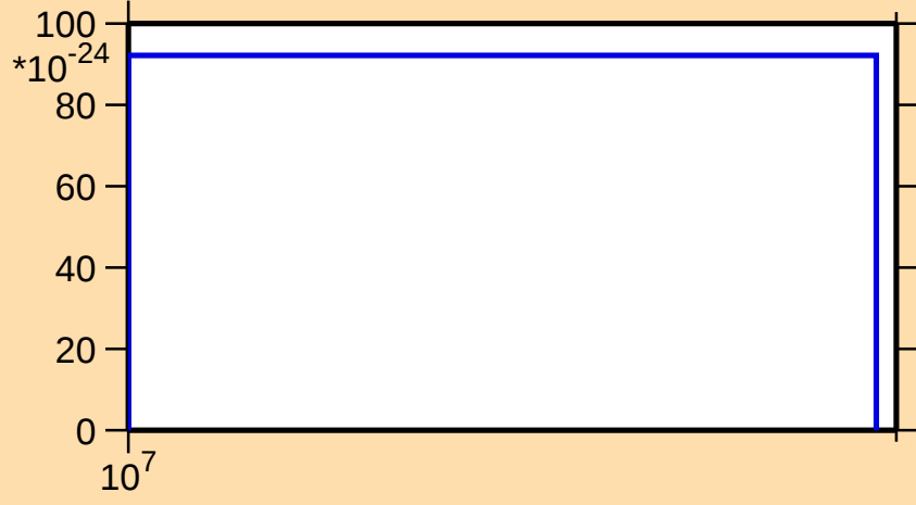
\sigma vs. E for ^{74}\text{Zn}(n,\text{nd})
