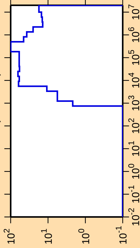
\Delta\sigma/\sigma vs. E for ^{74}\text{Zn}(n,\text{nonel.})
