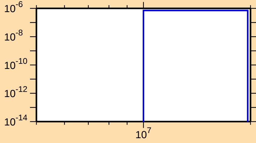
\sigma vs. E for ^{74}\text{Zn}(n,n\alpha)
