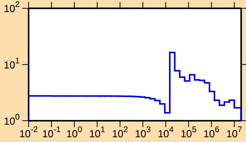
\sigma vs. E for ^{74}\text{Zn}(n,\text{el.})
