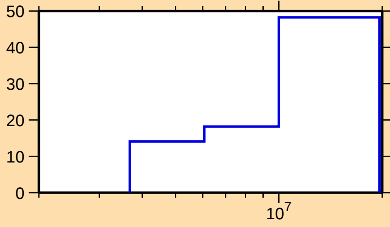
\Delta\sigma/\sigma vs. E for ^{74}\text{Zn}(n,\text{inel.})
