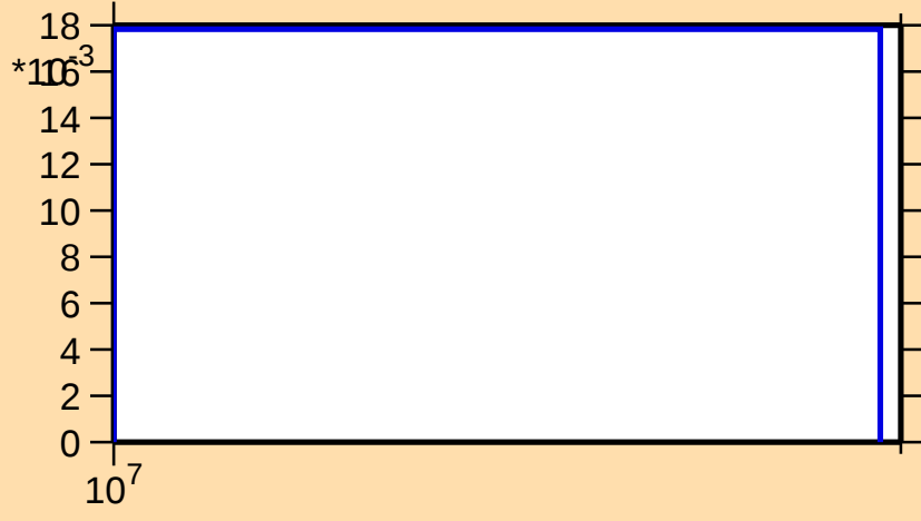
\sigma vs. E for ^{74}\text{Zn}(n,3n)
