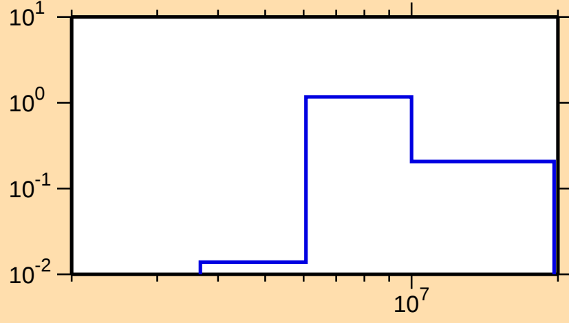
\sigma vs. E for ^{74}\text{Zn}(n,n\text{cont.})
