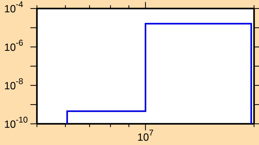
\sigma vs. E for ^{74}\text{Zn}(n,\alpha)
