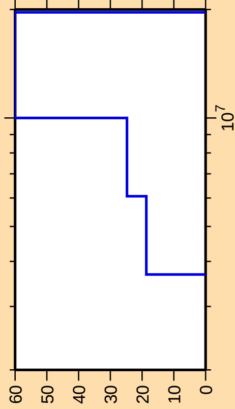
\Delta\sigma/\sigma vs. E for ^{74}\text{Zn}(n,n\text{cont.})
