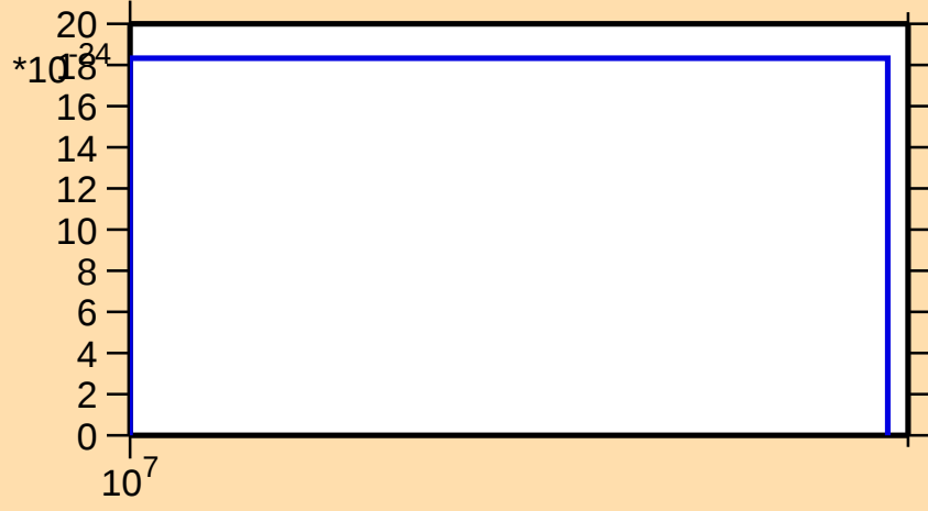
\sigma vs. E for ^{74}\text{Zn}(n,\text{He}3)
