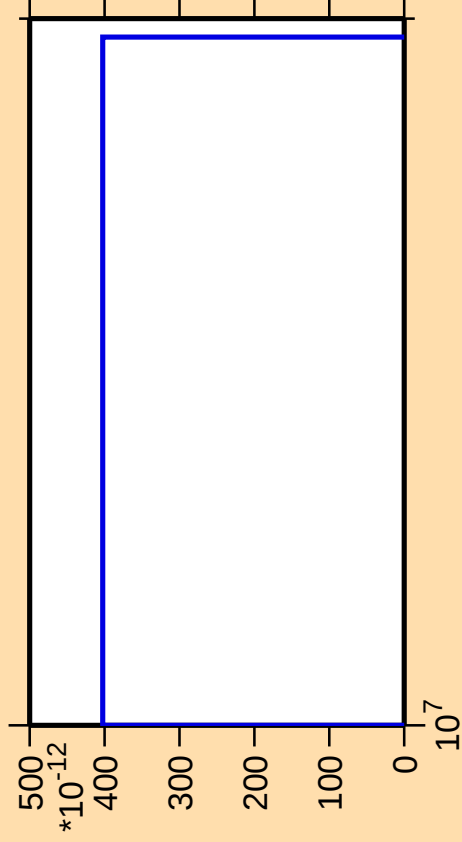
\Delta\sigma/\sigma vs. E for ^{74}\text{Zn}(n,\text{nd})
