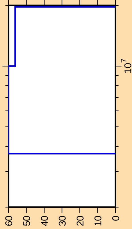
\Delta\sigma/\sigma vs. E for ^{74}\text{Zn}(n,\gamma)
