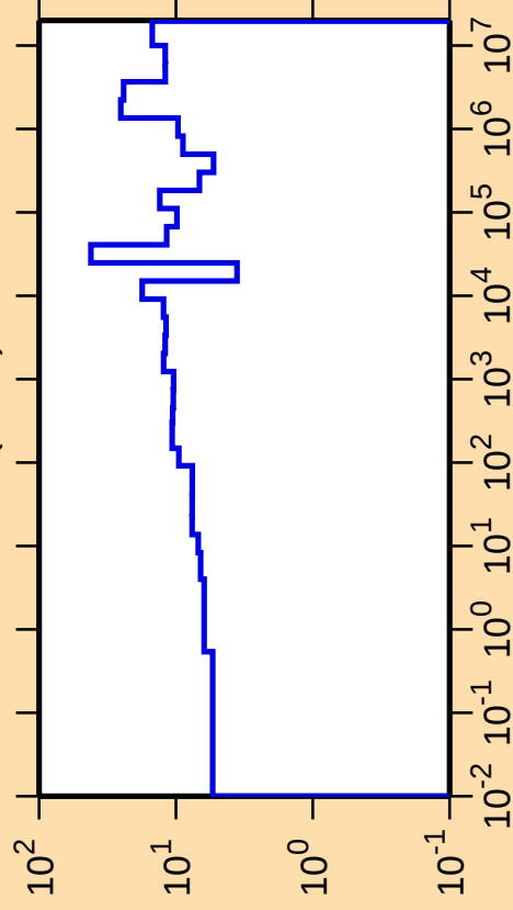
\Delta\sigma/\sigma vs. E for ^{74}\text{Zn}(n,\text{el.})
