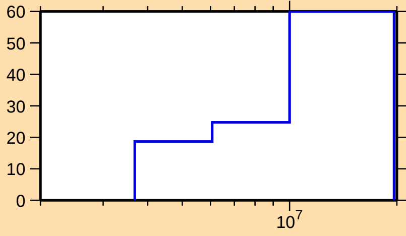
\Delta\sigma/\sigma vs. E for ^{74}\text{Zn}(n,n\text{cont.})
