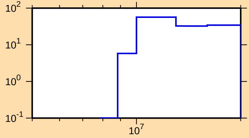
\Delta\sigma/\sigma vs. E for ^{77}\text{Zn}(n,p)
