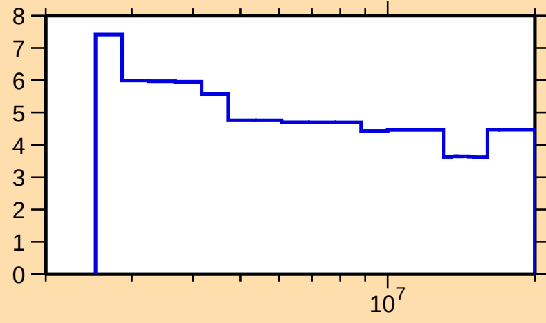
\Delta\sigma/\sigma vs. E for ^{77}\text{Zn}(\text{n},\text{nonel.})
