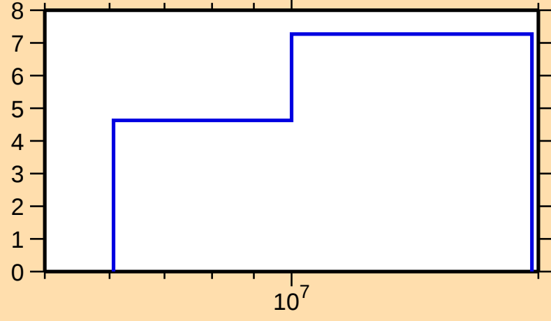
\Delta\sigma/\sigma vs. E for ^{77}\text{Zn}(n,2n)
