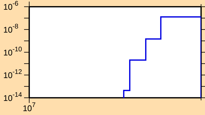
\sigma vs. E for ^{78}\text{Zn}(n,n\alpha)
