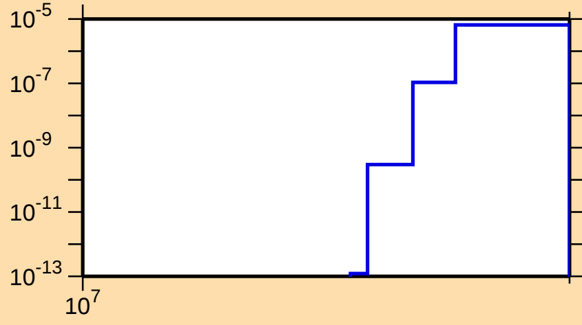
\sigma vs. E for ^{78}\text{Zn}(n,t)
