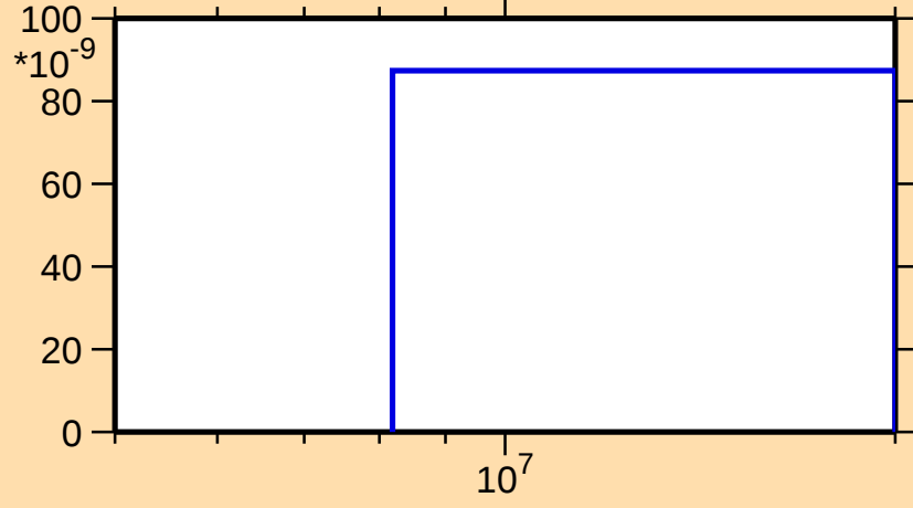
\sigma vs. E for ^{78}\text{Zn}(n,\alpha)
