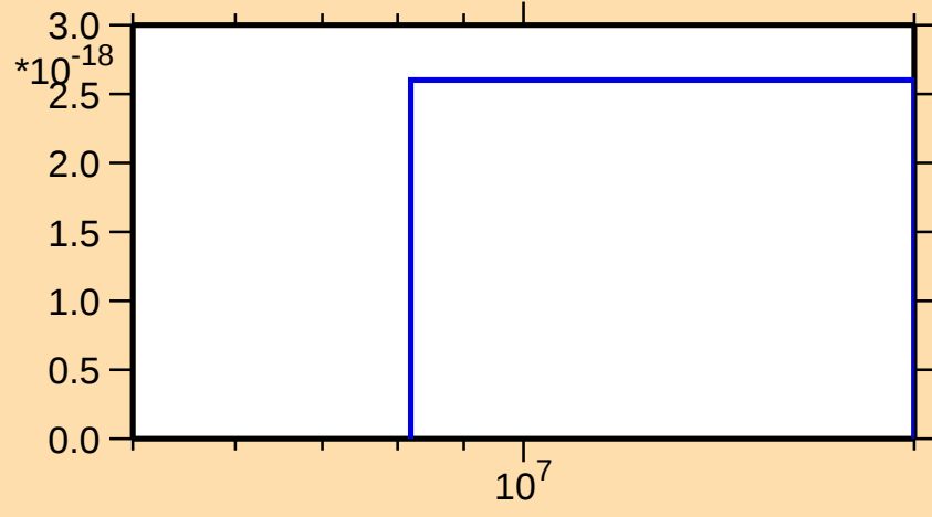
\sigma vs. E for ^{78}\text{Zn}(n,\text{nd})
