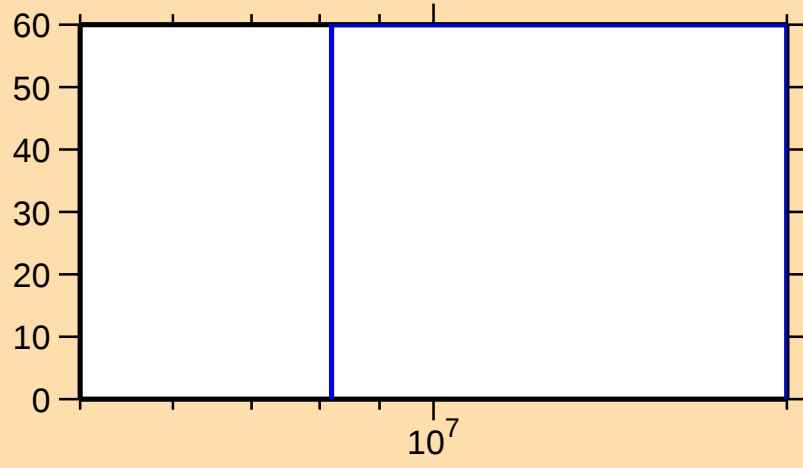
\Delta\sigma/\sigma vs. E for ^{78}\text{Zn}(n,\gamma)
