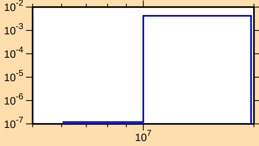
\sigma vs. E for ^{84}\text{Zr}(n,n\alpha)
