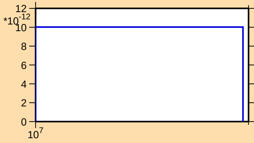
\sigma vs. E for ^{84}\text{Zr}(n,\text{pt})
