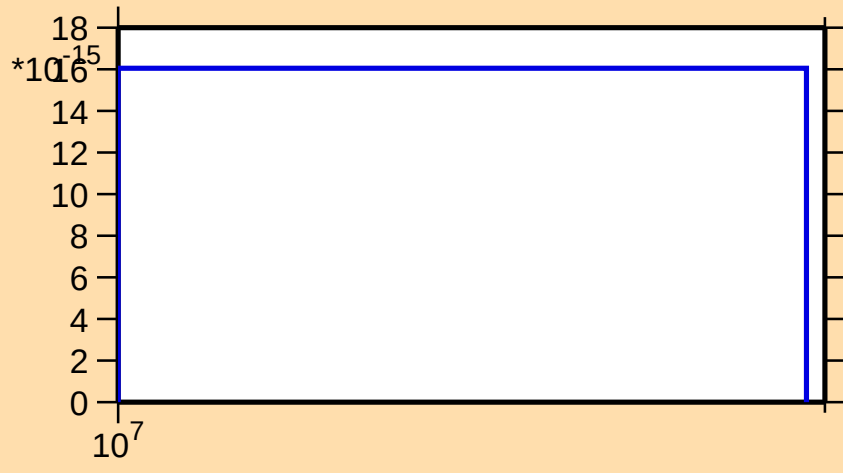
\sigma vs. E for ^{84}\text{Zr}(n,2np)
