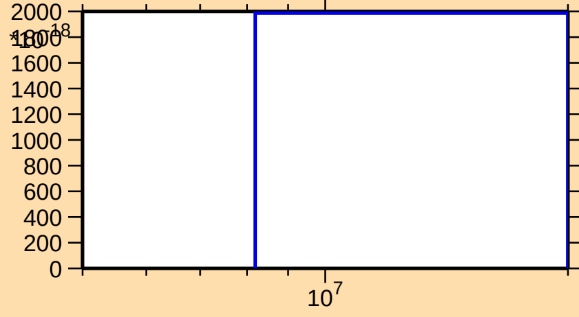
\sigma vs. E for ^{84}\text{Zr}(\text{mt } 34)
