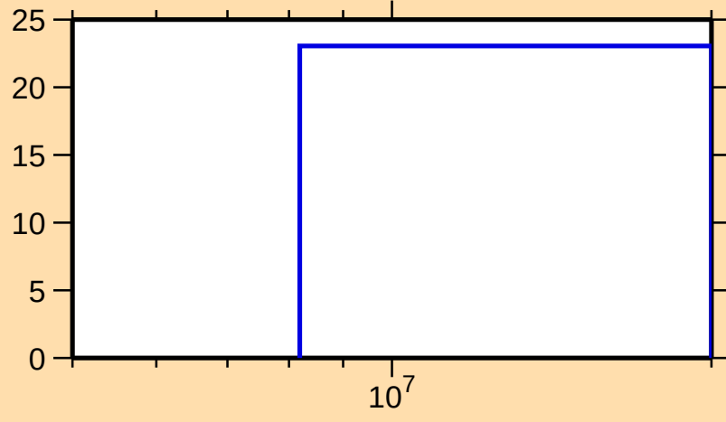
\Delta\sigma/\sigma vs. E for ^{84}\text{Zr}(n,\text{el.})
