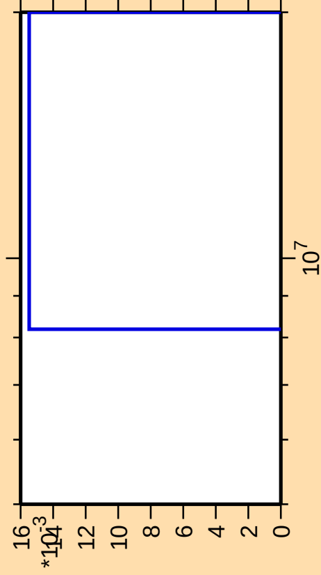
\Delta\sigma/\sigma vs. E for ^{84}\text{Zr}(\text{mt } 34)
