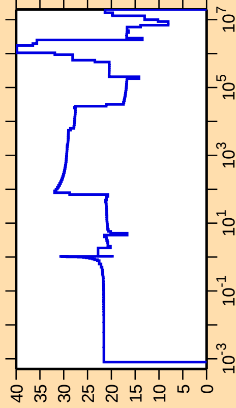
\Delta\sigma/\sigma vs. E for ^{85}\text{Zr}(n,\text{el.})
