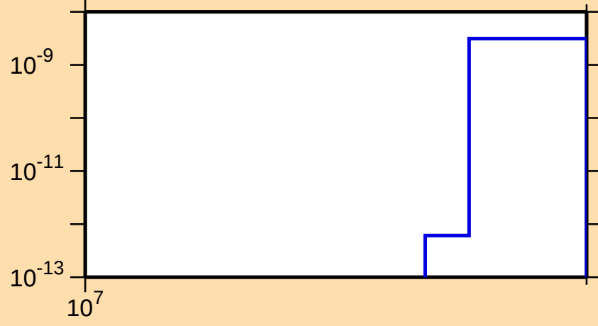
\sigma vs. E for ^{85}\text{Zr}(\text{mt } 45)
