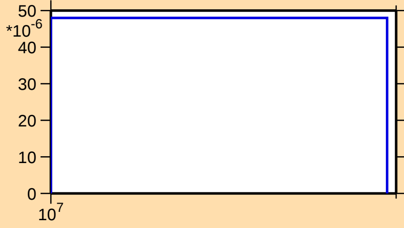
\sigma vs. E for ^{85}\text{Zr}(n,\text{pd})
