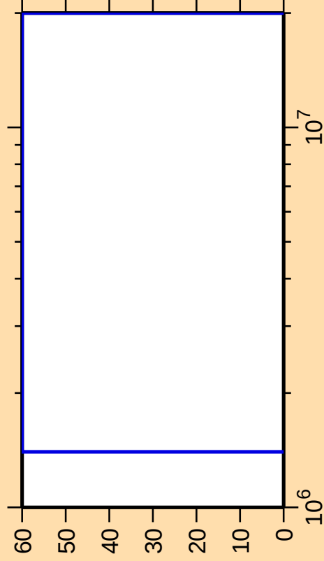
\Delta\sigma/\sigma vs. E for ^{85}\text{Zr}(\text{n},\text{ncont.})
