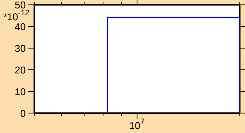
\sigma vs. E for ^{85}\text{Zr}(\text{mt } 34)
