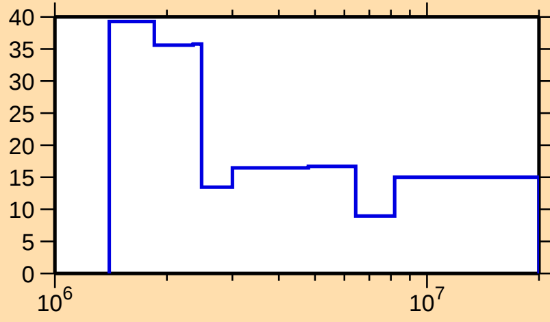
\Delta\sigma/\sigma vs. E for ^{85}\text{Zr}(\text{n},\text{el.})
