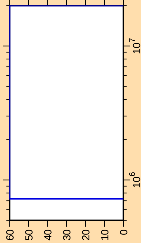
\Delta\sigma/\sigma vs. E for ^{86}\text{Zr}(n,\alpha)
