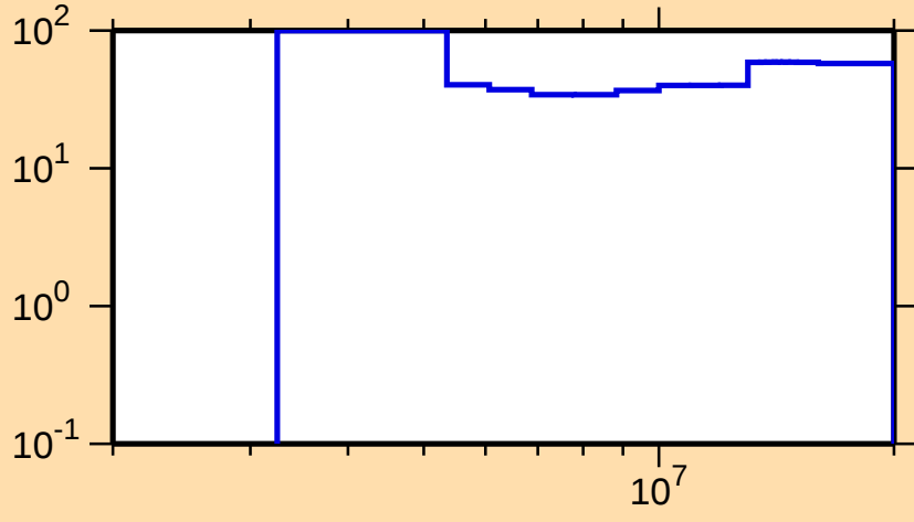
\Delta\sigma/\sigma vs. E for ^{86}\text{Zr}(n,n\text{cont.})
