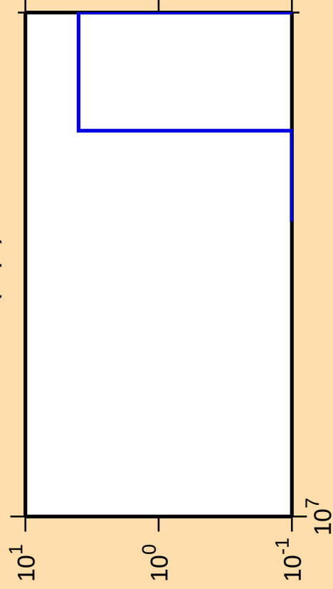
\Delta\sigma/\sigma vs. E for ^{86}\text{Zr}(n,\text{pt})
