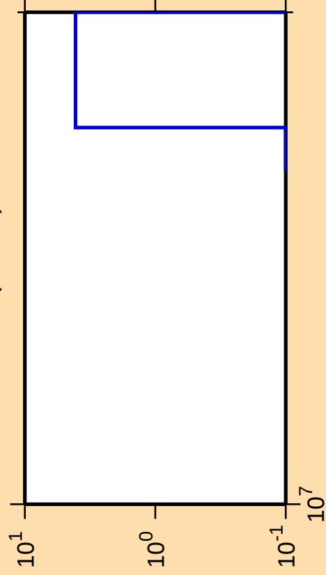
\Delta\sigma/\sigma vs. E for ^{86}\text{Zr}(\text{mt 45})
