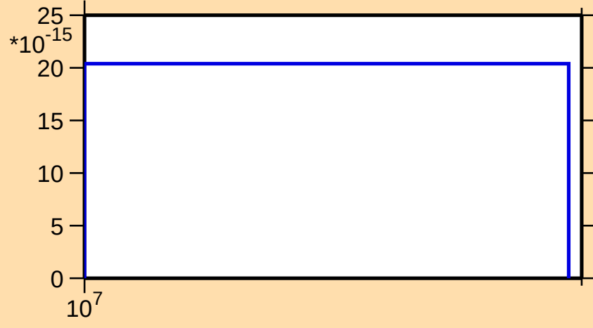
\sigma vs. E for ^{86}\text{Zr} (mt 45)
