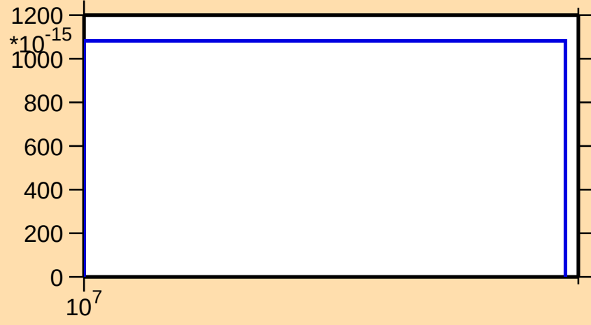
\sigma vs. E for ^{86}\text{Zr}(n,\text{nd})
