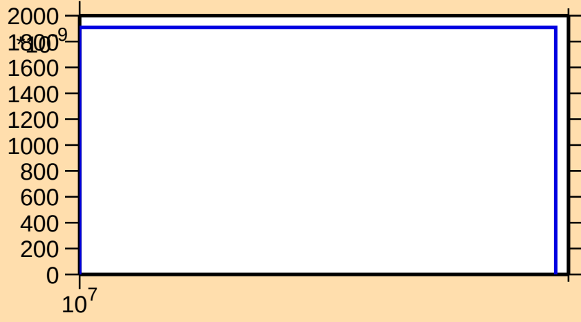
\sigma vs. E for ^{86}\text{Zr}(n,t)
