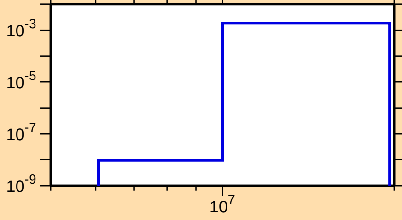
\sigma vs. E for ^{86}\text{Zr}(n,n\alpha)
