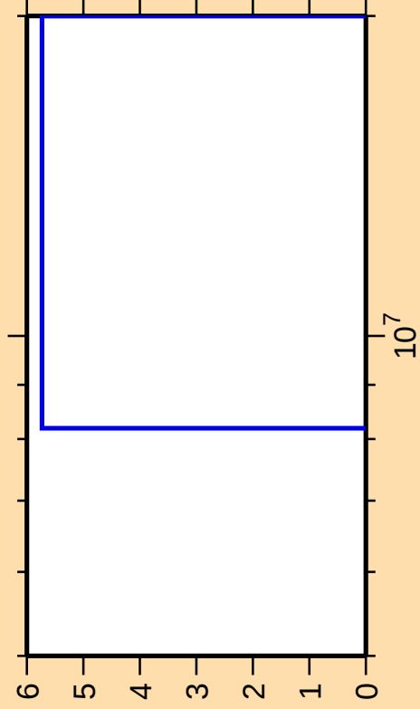
\Delta\sigma/\sigma vs. E for ^{86}\text{Zr}(n,\text{nd})
