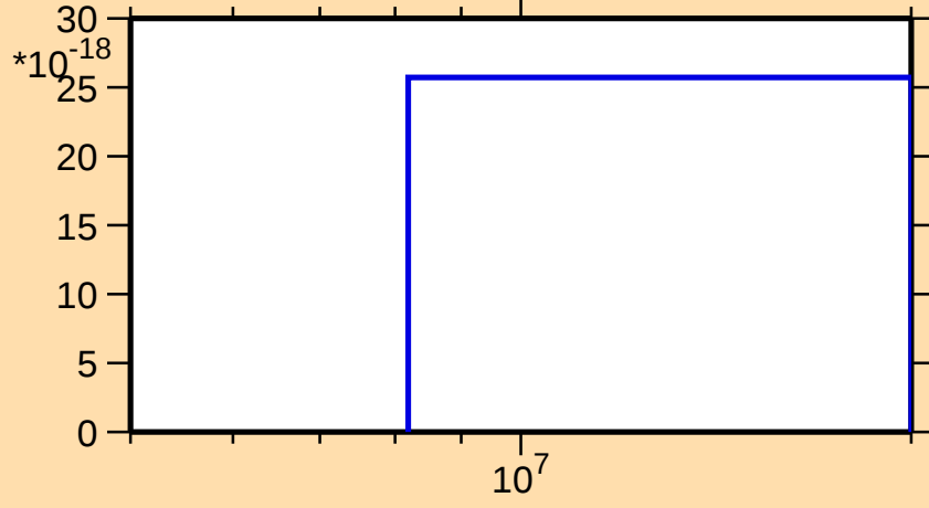
\sigma vs. E for ^{86}\text{Zr}(n,2np)
