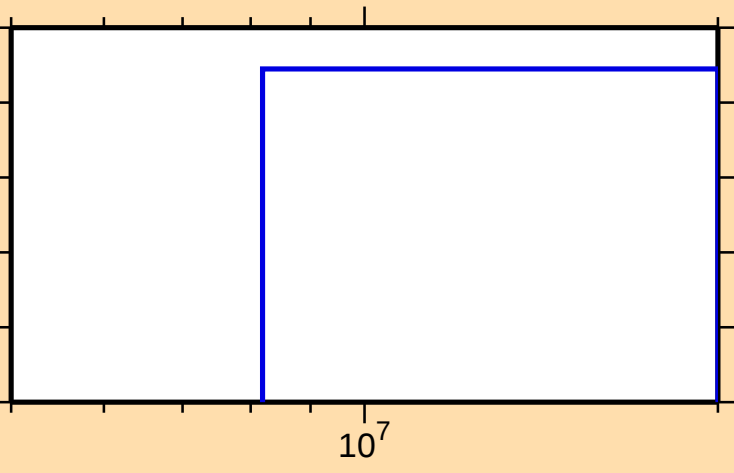
\sigma vs. E for ^{86}\text{Zr}(n,\text{pd})
