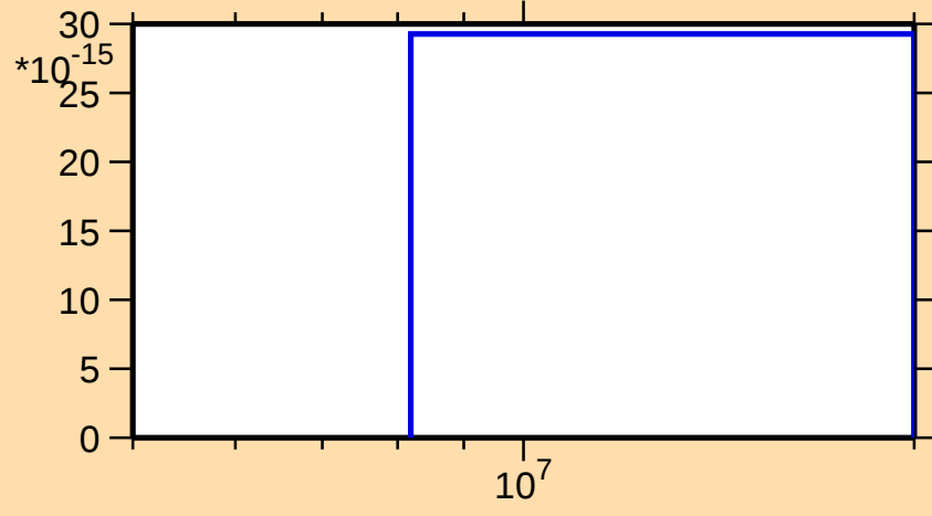
\sigma vs. E for ^{86}\text{Zr}(\text{mt } 45)
