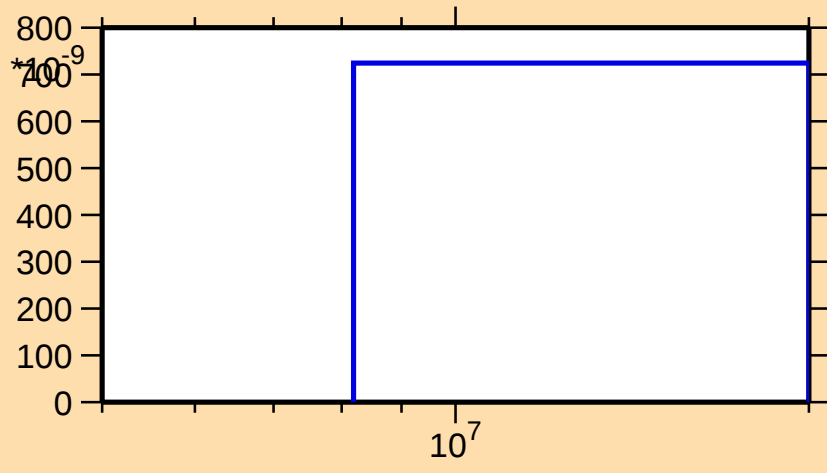
\sigma vs. E for ^{86}\text{Zr}(n,\text{He3})
