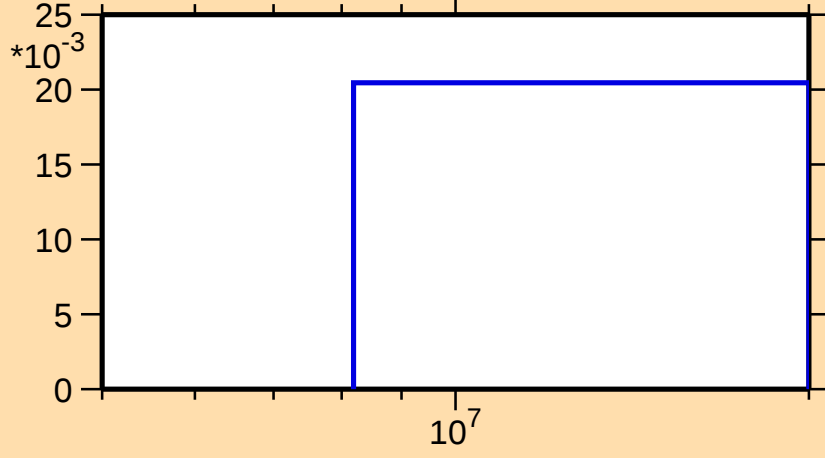
\sigma vs. E for ^{86}\text{Zr}(n,2n)
