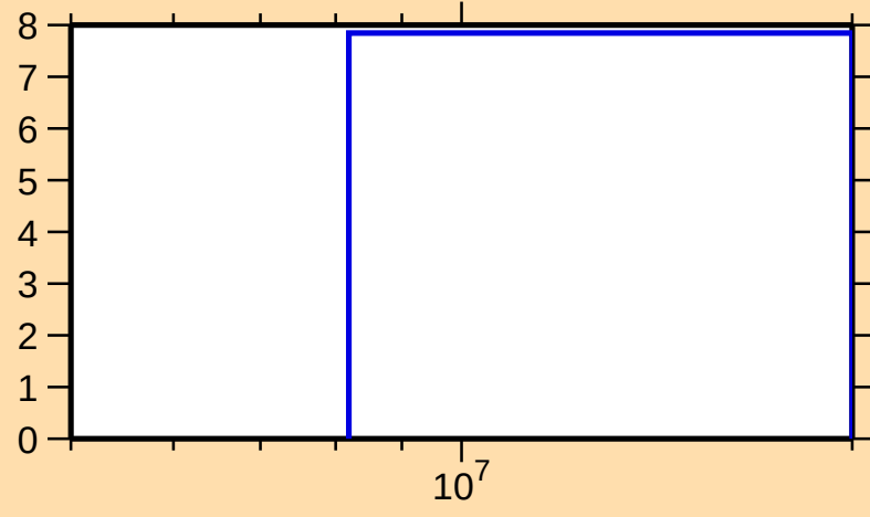
\Delta\sigma/\sigma vs. E for ^{88}\text{Zr}(n,\text{inel.})
