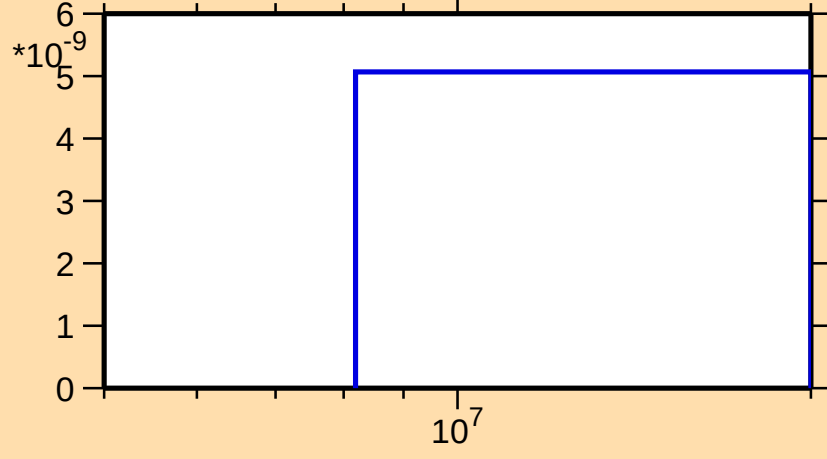
\sigma vs. E for ^{88}\text{Zr}(n,\text{pd})
