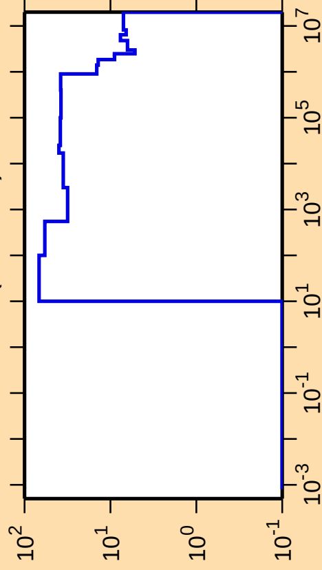
\Delta\sigma/\sigma vs. E for ^{88}\text{Zr}(n,\text{nonel.})
