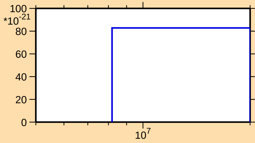
\sigma vs. E for ^{88}\text{Zr}(n,2np)
