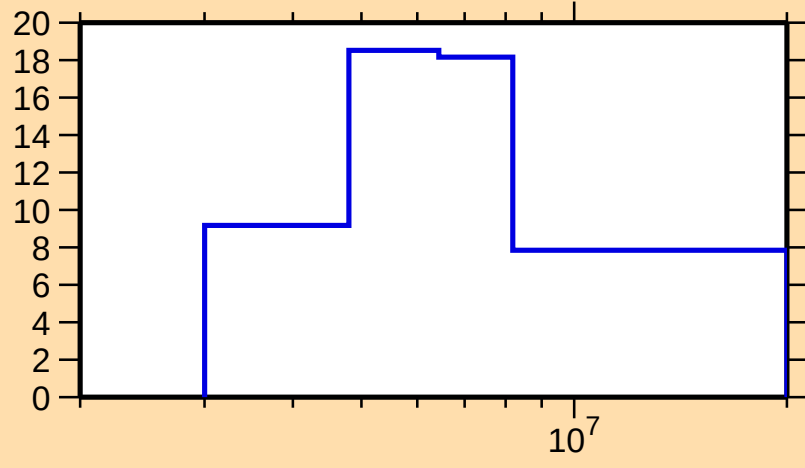
\Delta\sigma/\sigma vs. E for ^{88}\text{Zr}(\text{n},\text{inel.})
