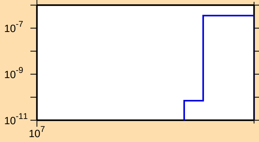
\sigma vs. E for ^{99}\text{Zr}(n,nt)
