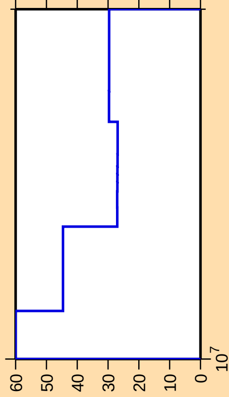
\Delta\sigma/\sigma vs. E for ^{99}\text{Zr}(n,3n)
