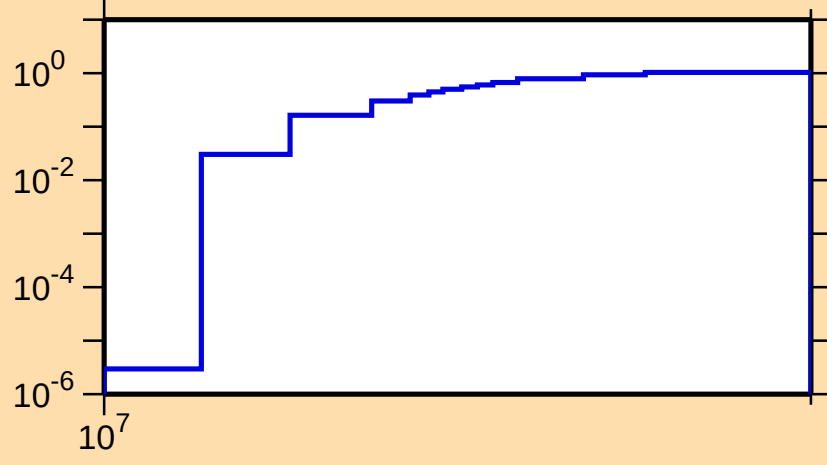
\sigma vs. E for ^{99}\text{Zr}(n,3n)
