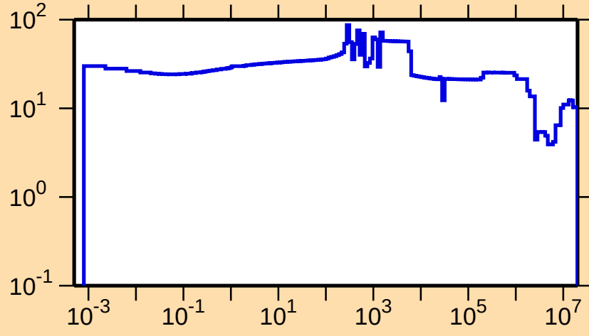
\Delta\sigma/\sigma vs. E for ^{99}\text{Zr}(n,\text{tot.})
