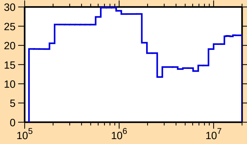
\Delta\sigma/\sigma vs. E for ^{99}\text{Zr}(n,\text{el.})
