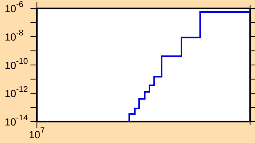
\sigma vs. E for ^{99}\text{Zr}(n,2n\alpha)
