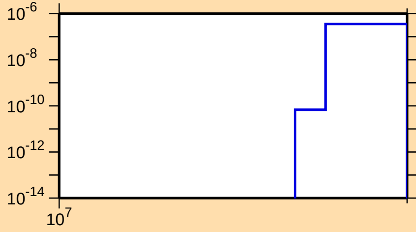
\sigma vs. E for ^{99}\text{Zr}(n,\text{nd})
