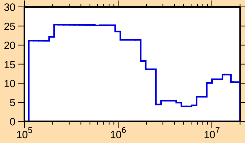
\Delta\sigma/\sigma vs. E for ^{99}\text{Zr}(n,\text{tot.})
