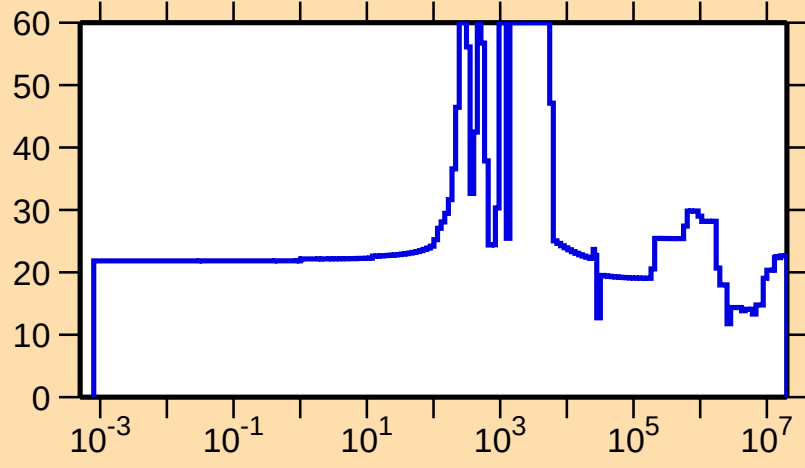
\Delta\sigma/\sigma vs. E for ^{99}\text{Zr}(n,\text{el.})
