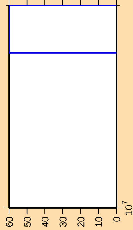
\Delta\sigma/\sigma vs. E for ^{99}\text{Zr}(n,2np)
