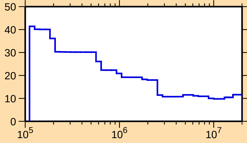
\Delta\sigma/\sigma vs. E for ^{99}\text{Zr}(n,\text{nonel.})
