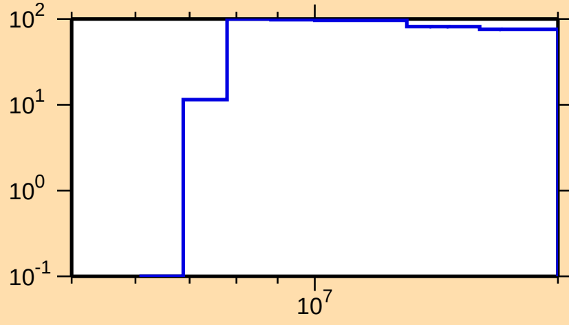
\Delta\sigma/\sigma vs. E for ^{99}\text{Zr}(n,p)
