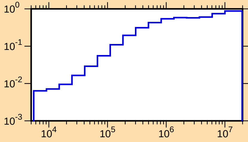
\mu vs. E for ^{99}\text{Zr}(\text{mt251})
