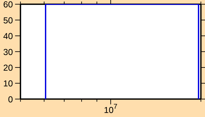
\Delta\sigma/\sigma vs. E for ^{99}\text{Zr}(n,\text{inel.})
