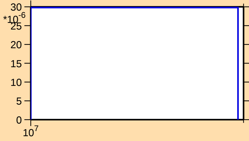
\sigma vs. E for ^{99}\text{Zr}(n,d)
