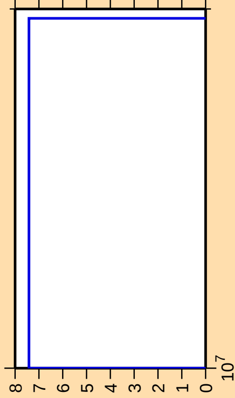
\Delta\sigma/\sigma vs. E for ^{99}\text{Zr}(n,2np)
