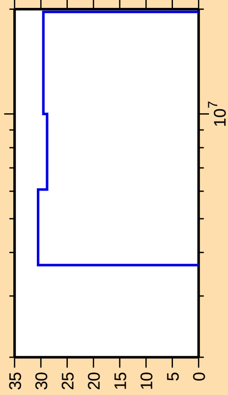
\Delta\sigma/\sigma vs. E for ^{99}\text{Zr}(n,2n)
