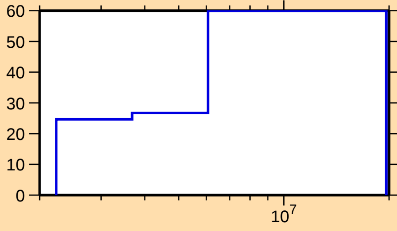
\Delta\sigma/\sigma vs. E for ^{99}\text{Zr}(n,n\text{cont.})
