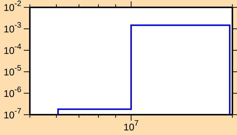
\sigma vs. E for ^{99}\text{Zr}(n,p)
