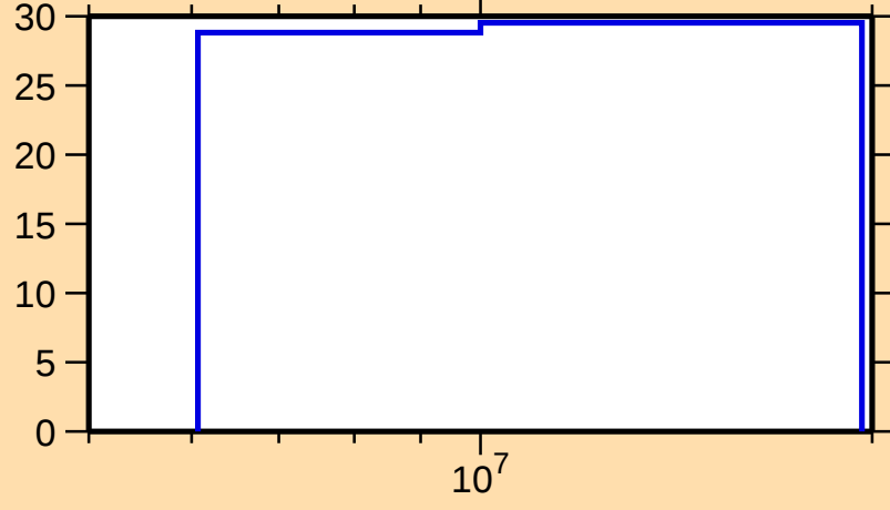
\Delta\sigma/\sigma vs. E for ^{99}\text{Zr}(n,2n)
