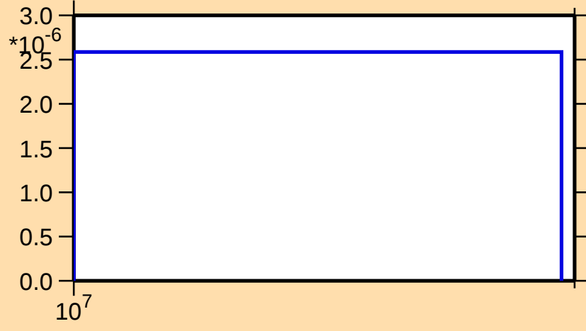
\sigma vs. E for ^{99}\text{Zr}(n,np)
