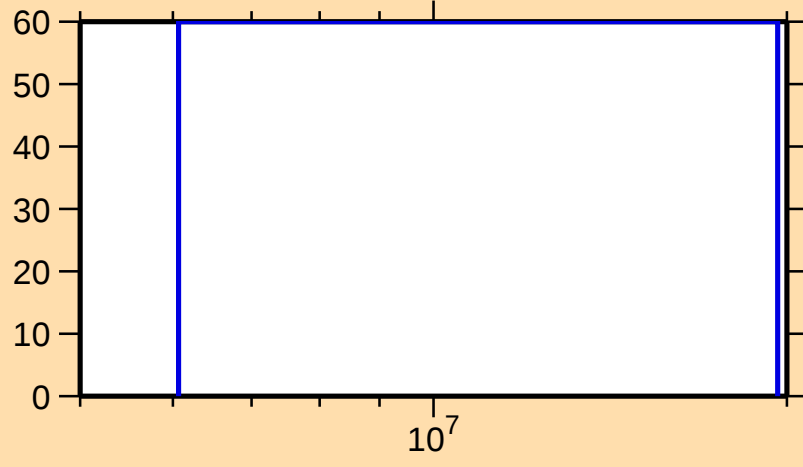
\Delta\sigma/\sigma vs. E for ^{99}\text{Zr}(n,n\text{cont.})
