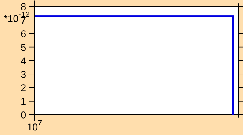
\sigma vs. E for ^{99}\text{Zr}(n,2np)
