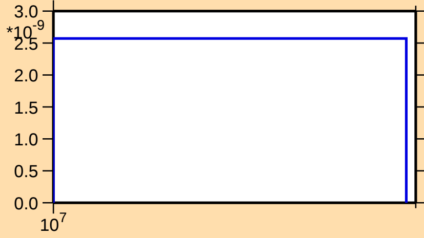
\sigma vs. E for ^{99}\text{Zr}(n,\text{nd})
