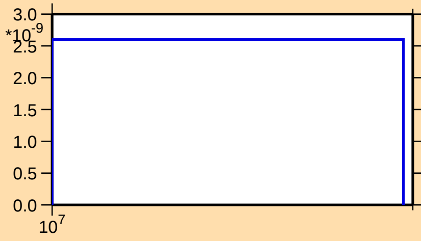
\sigma vs. E for ^{99}\text{Zr}(n,\text{nt})
