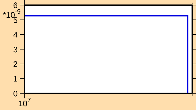
\sigma vs. E for ^{99}\text{Zr}(n,2n\alpha)
