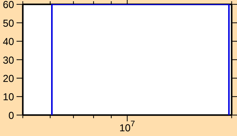
\Delta\sigma/\sigma vs. E for ^{99}\text{Zr}(n,\gamma)
