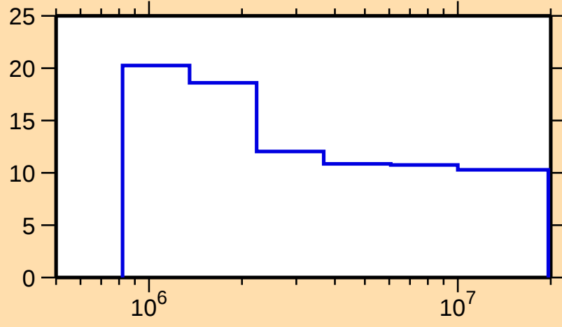
\Delta\sigma/\sigma vs. E for ^{99}\text{Zr}(\text{n},\text{nonel.})
