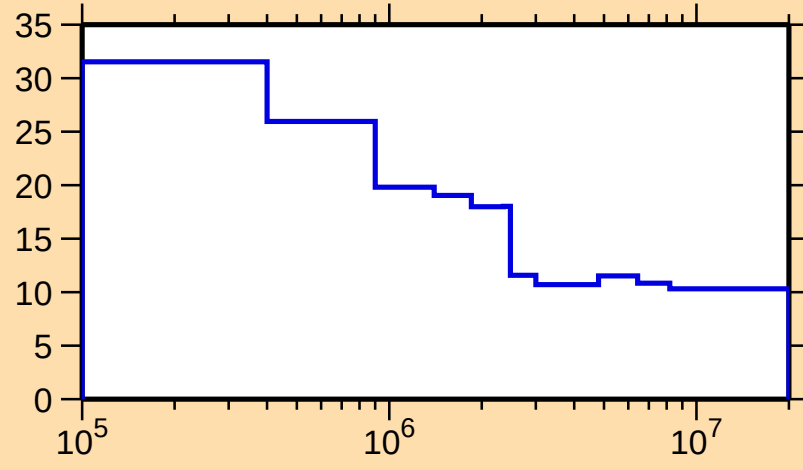
\Delta\sigma/\sigma vs. E for ^{99}\text{Zr}(n,\text{nonel.})
