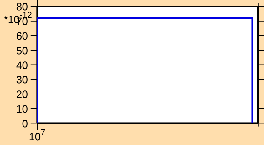
\sigma vs. E for ^{104}\text{Ag}(\text{mt } 45)
