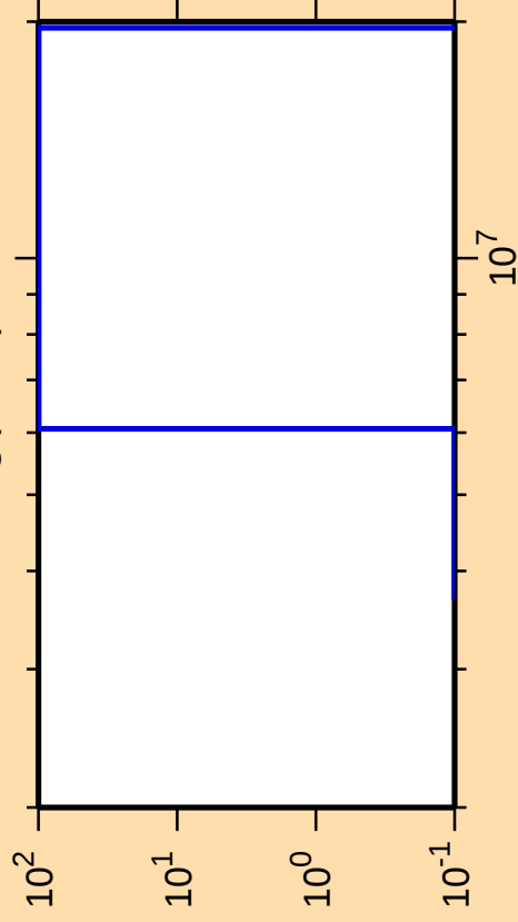
\Delta\sigma/\sigma vs. E for ^{104}\text{Ag}(n,n\alpha)
