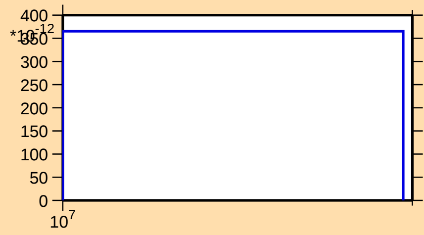
\sigma vs. E for ^{104}\text{Ag}(n,\text{nt})
