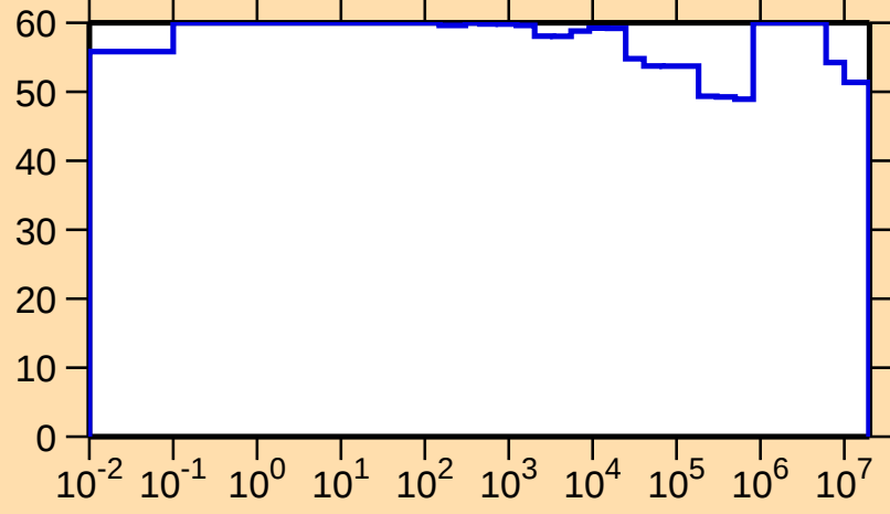
\Delta\sigma/\sigma vs. E for ^{104}\text{Ag}(n,p)
