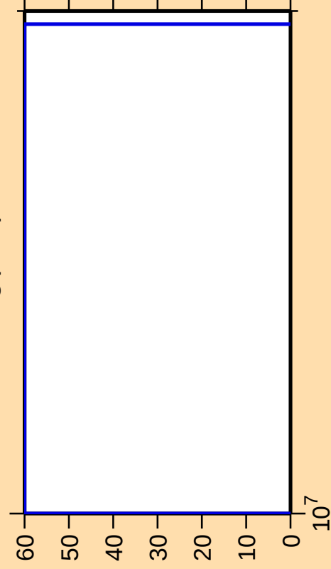
\Delta\sigma/\sigma vs. E for ^{104}\text{Ag}(n,\text{nt})
