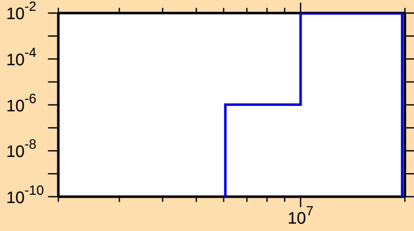
\sigma vs. E for ^{104}\text{Ag}(n,n\alpha)
