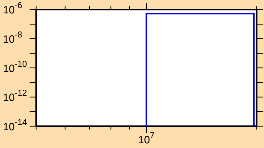
\sigma vs. E for ^{104}\text{Ag}(n,\text{He3})
