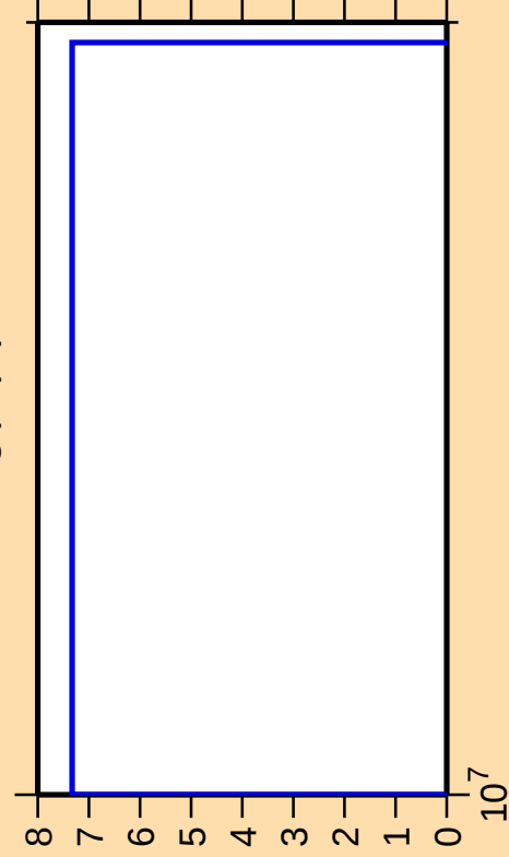
\Delta\sigma/\sigma vs. E for ^{104}\text{Ag}(n,\text{pt})
