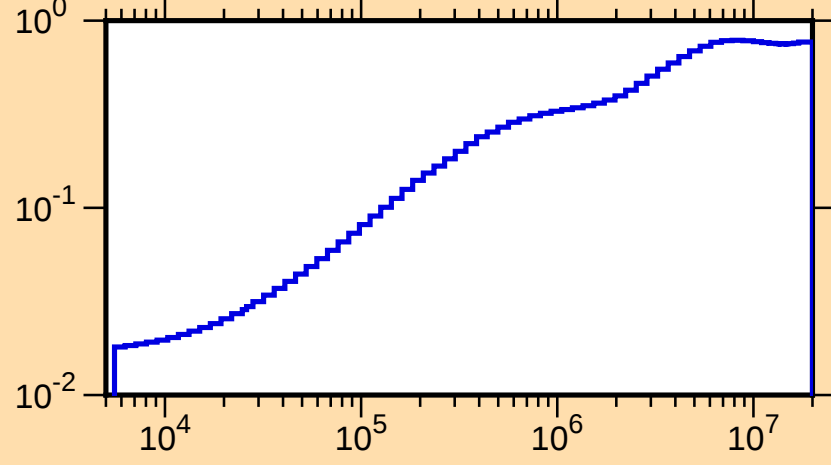
\mu vs. E for ^{41}\text{Ar}(\text{mt251})
