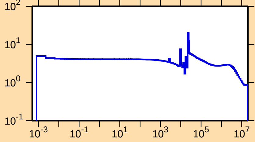
\sigma vs. E for ^{41}\text{Ar}(n,\text{el.})
