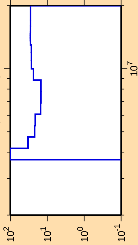
\Delta\sigma/\sigma vs. E for ^{41}\text{Ar}(n,\text{ncont.})
